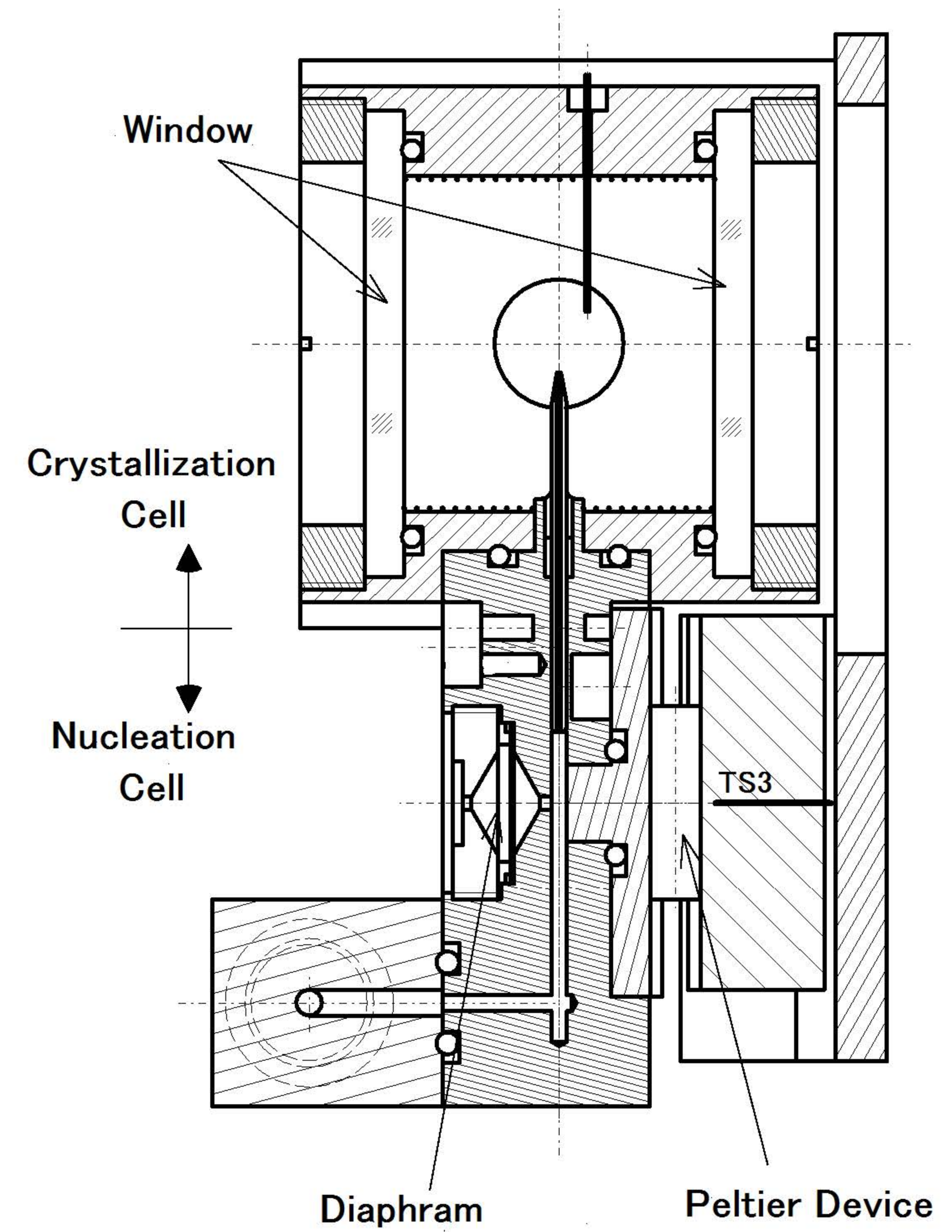
General Drawing of ICE-CELL ( Crystallization Cell and Nucleation cell )
