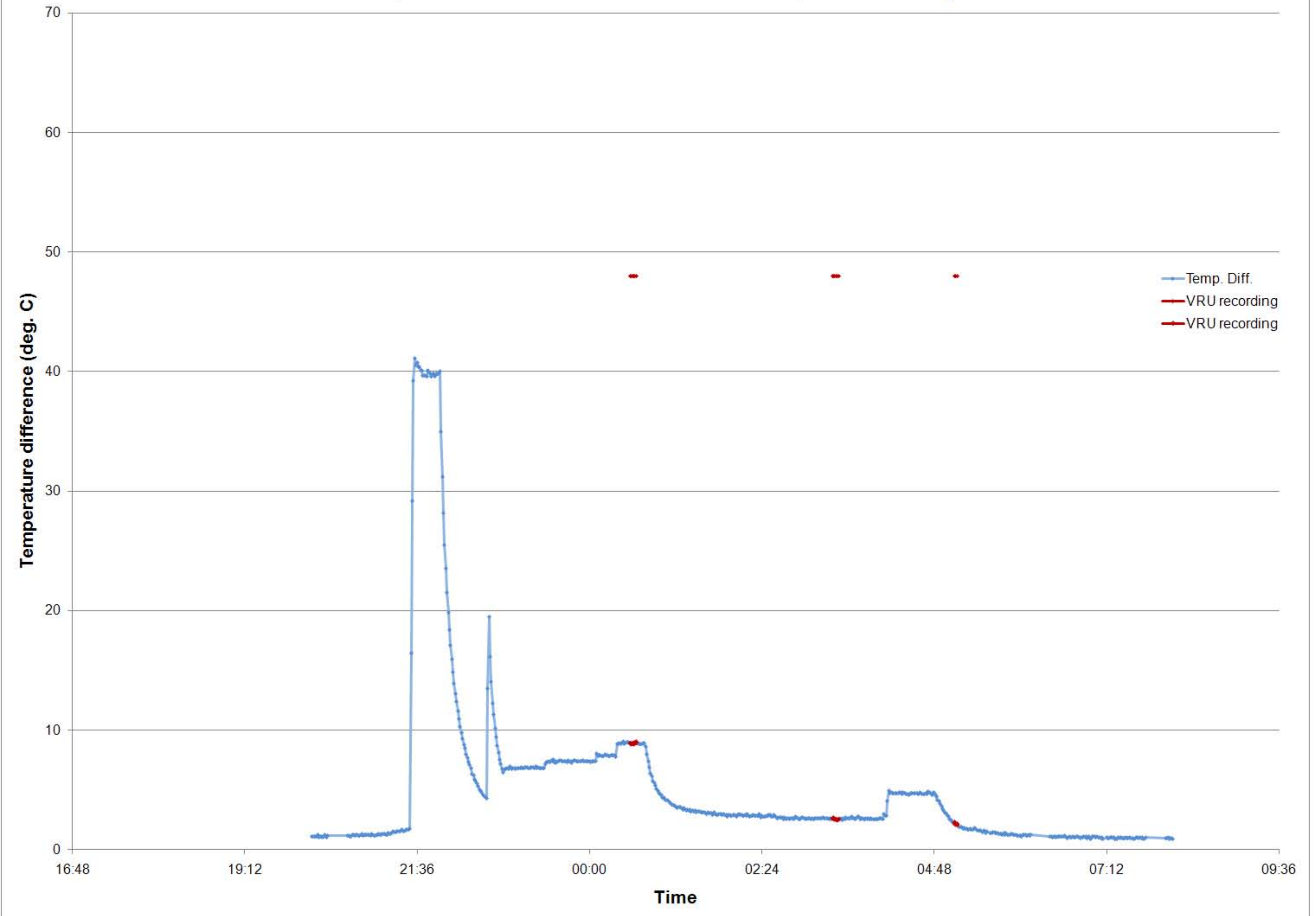
MEIS2-07 Temperatrure difference between HD and CD, VRU recording
