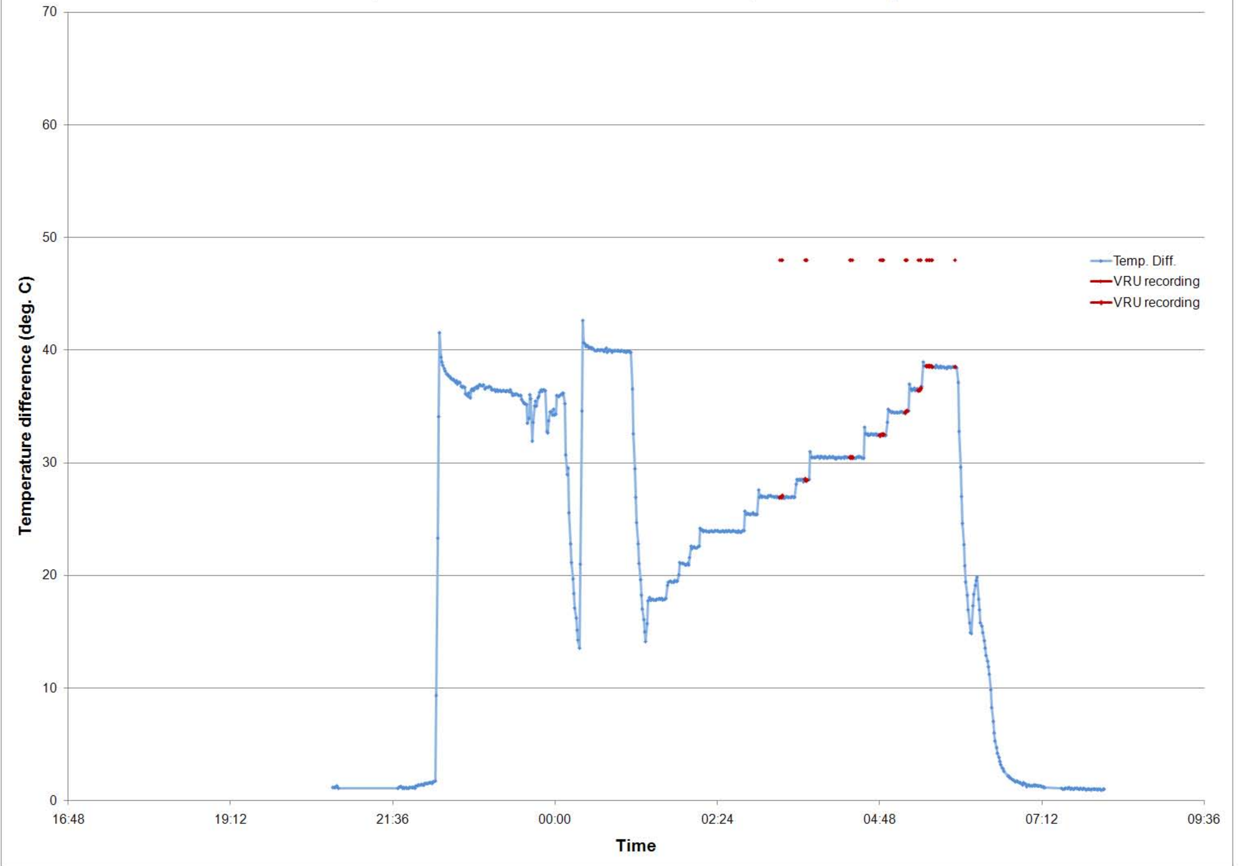
MEIS2-03 Temperatrure difference between HD and CD, VRU recording
