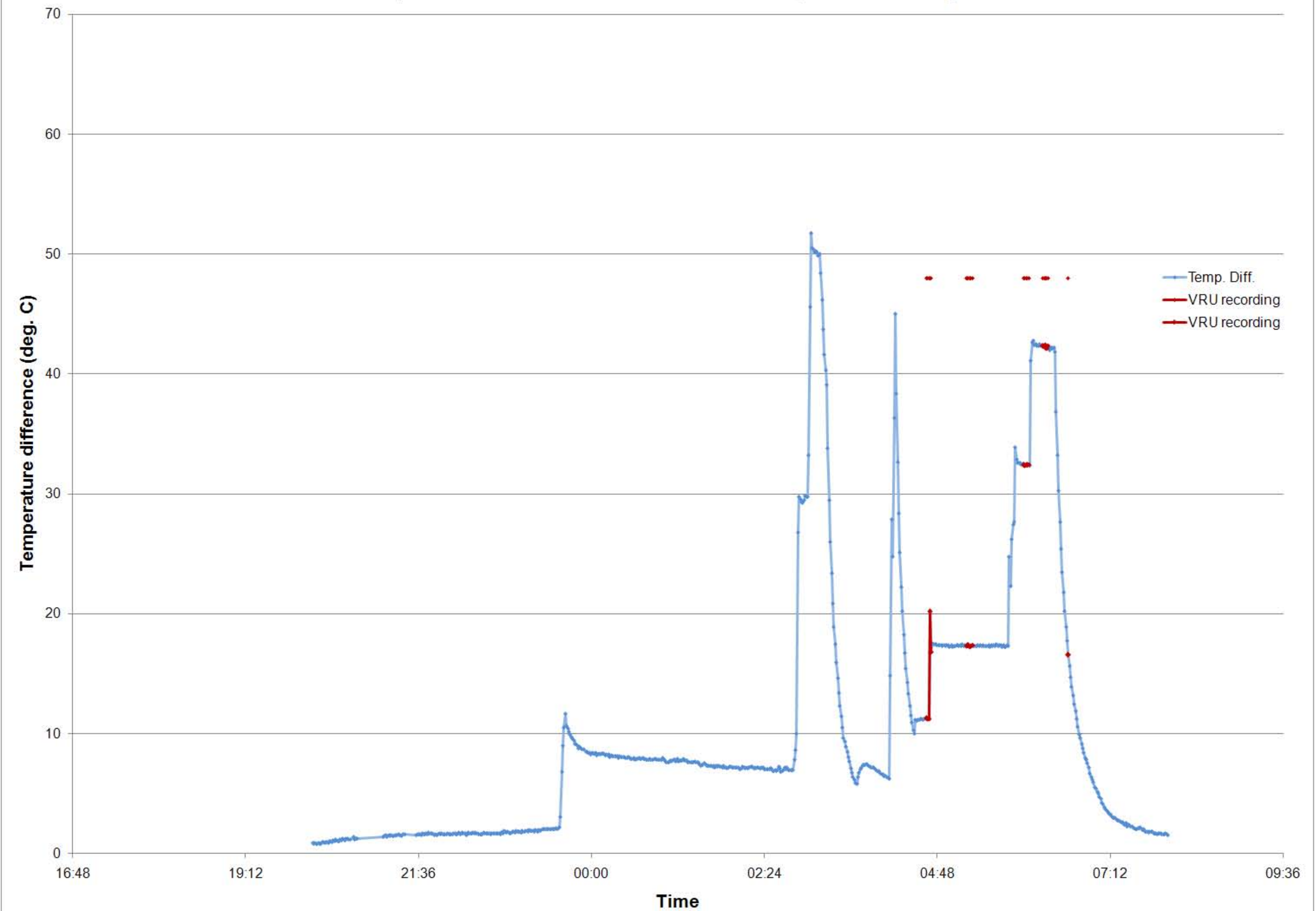
MEIS2-01 Temperatrure difference between HD and CD, VRU recording
