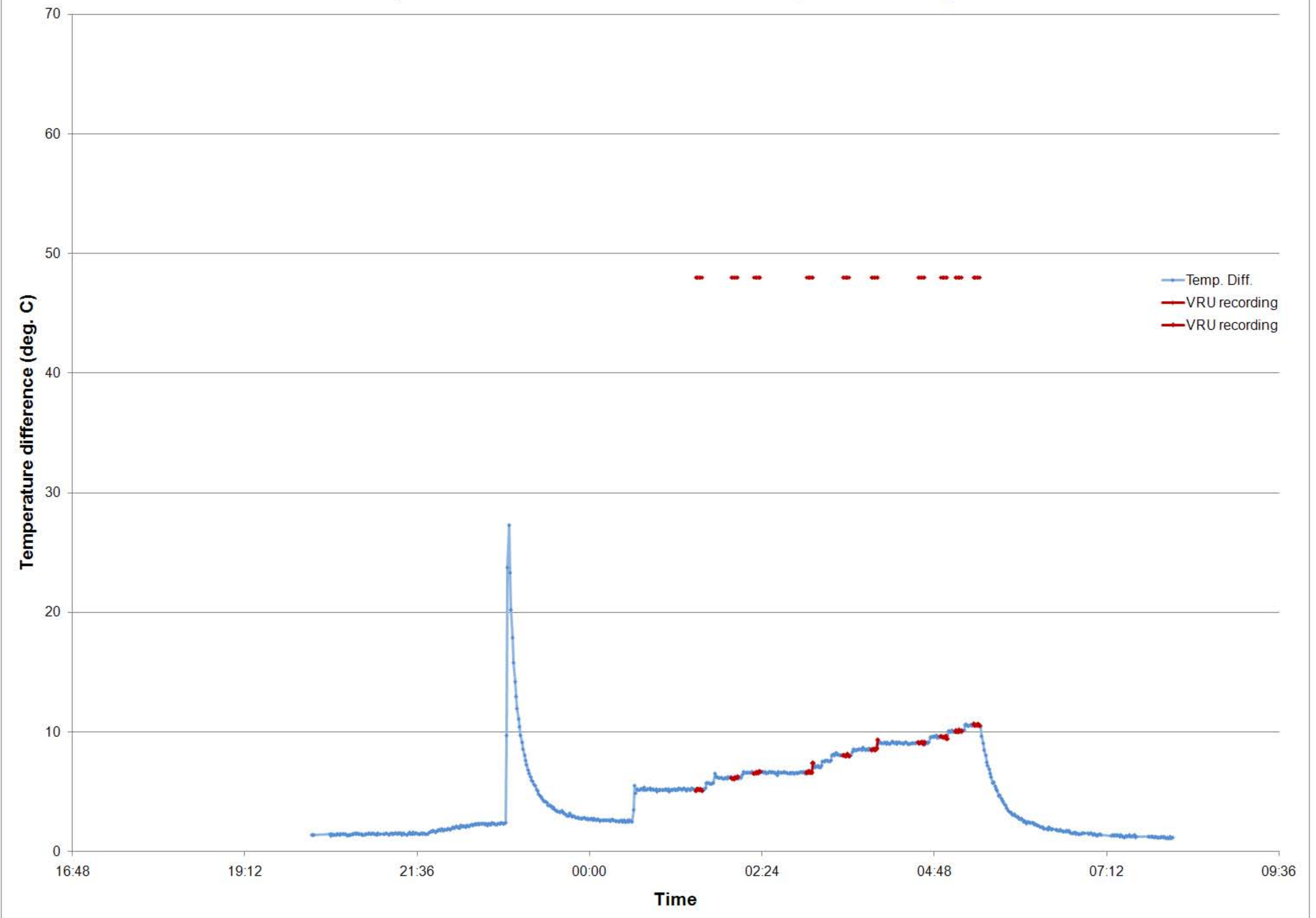
MEIS2-02 Temperatrure difference between HD and CD, VRU recording
