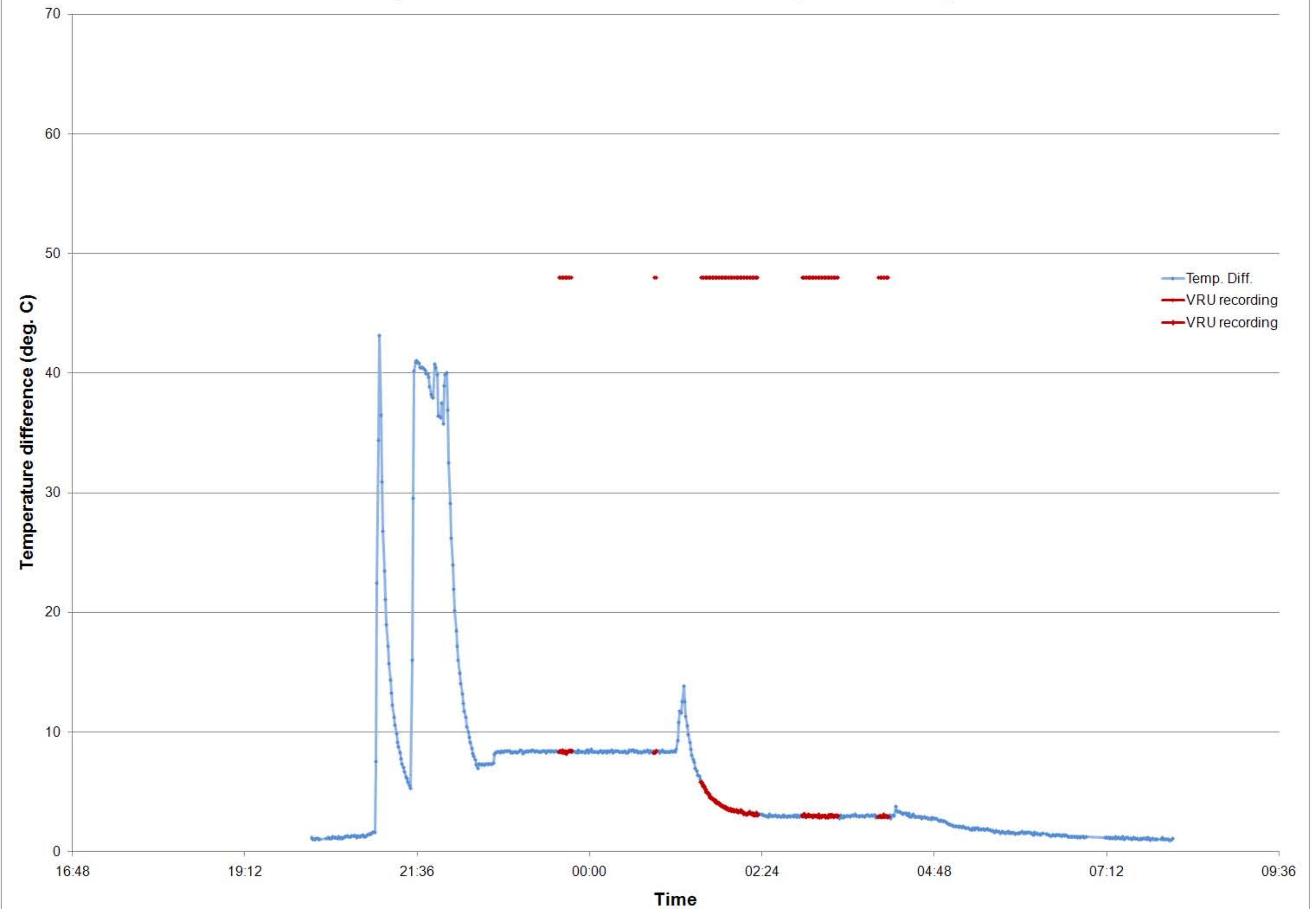
MEIS2-06 Temperatrure difference between HD and CD, VRU recording
