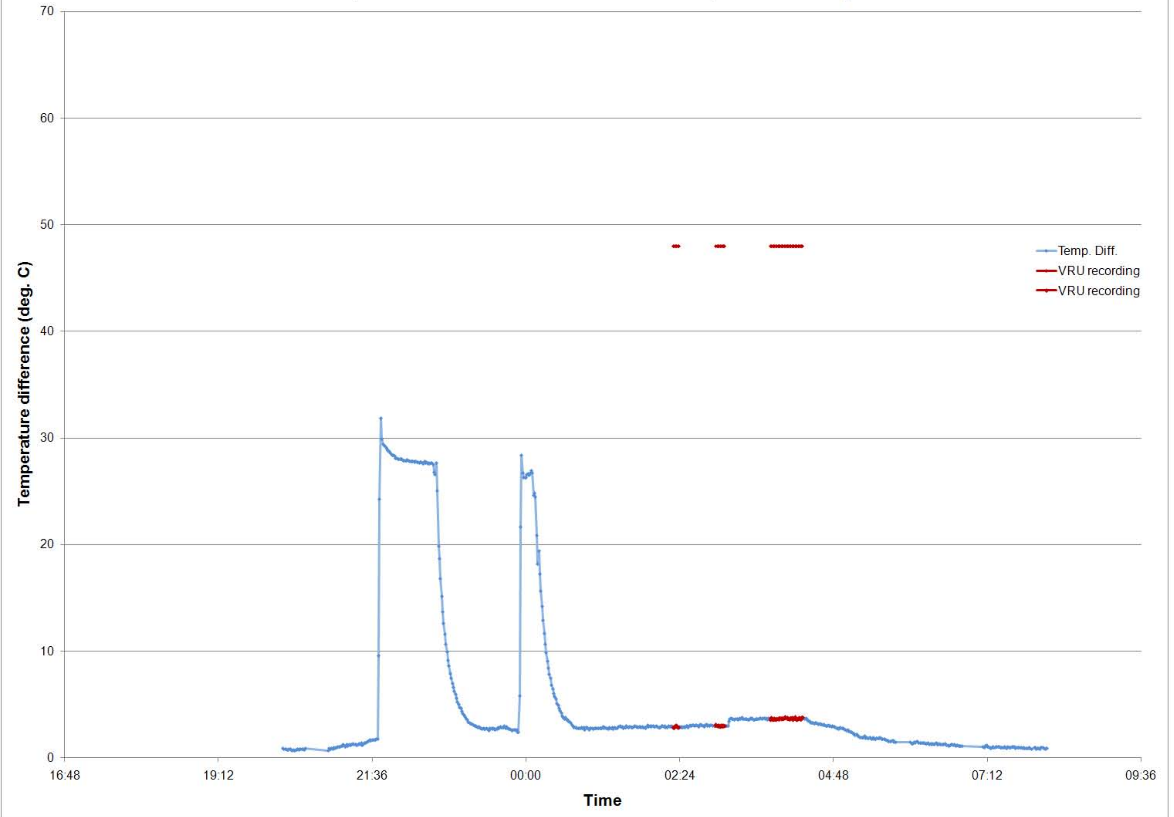
MEIS2-12 Temperatrure difference between HD and CD, VRU recording
