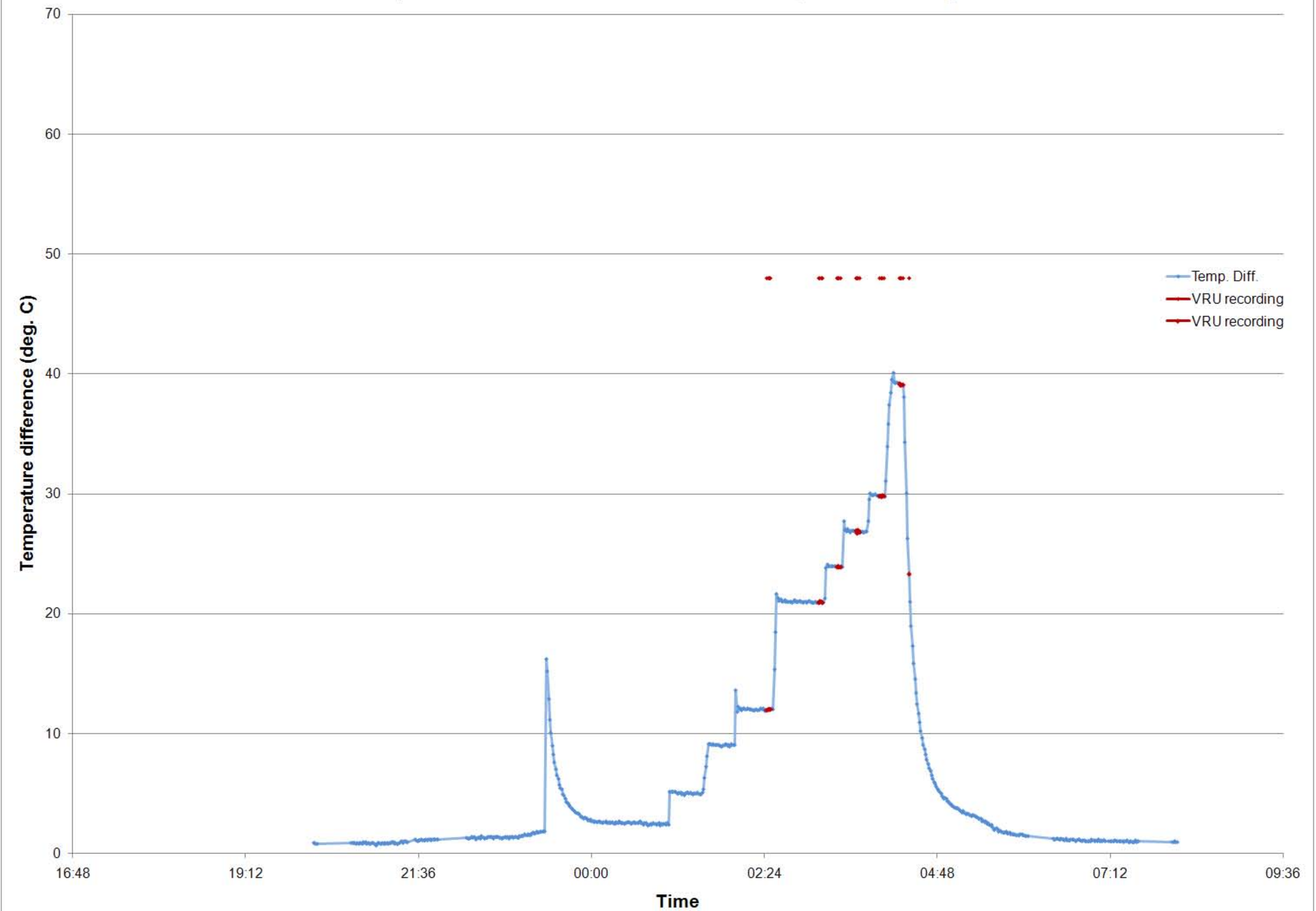
MEIS2-14 Temperatrure difference between HD and CD, VRU recording
