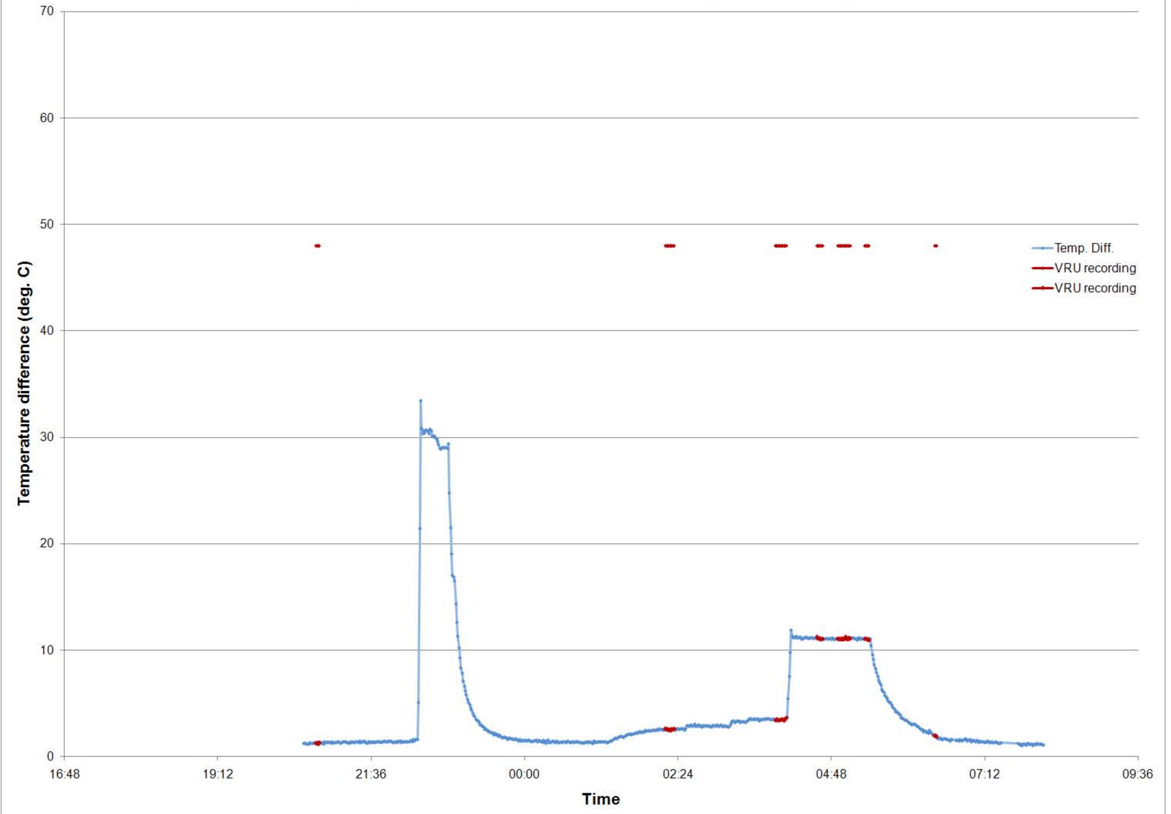
MEIS2-09 Temperatrure difference between HD and CD, VRU recording
