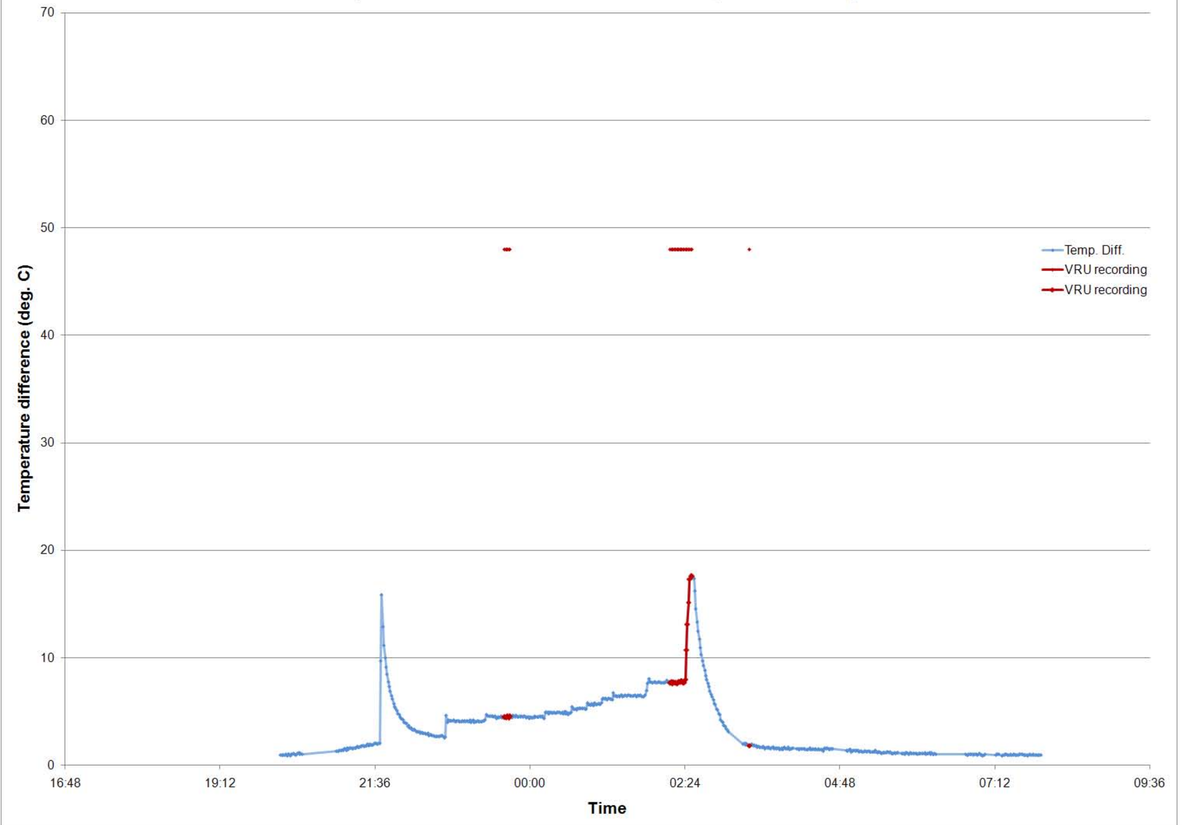
MEIS2-10 Temperatrure difference between HD and CD, VRU recording
