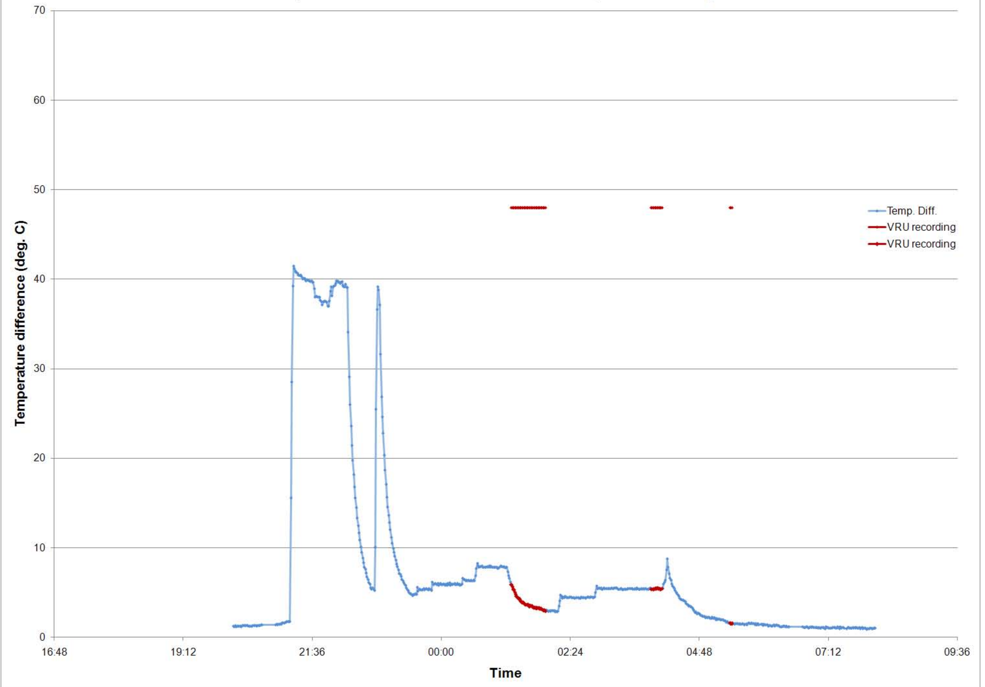
MEIS2-05 Temperatrure difference between HD and CD, VRU recording
