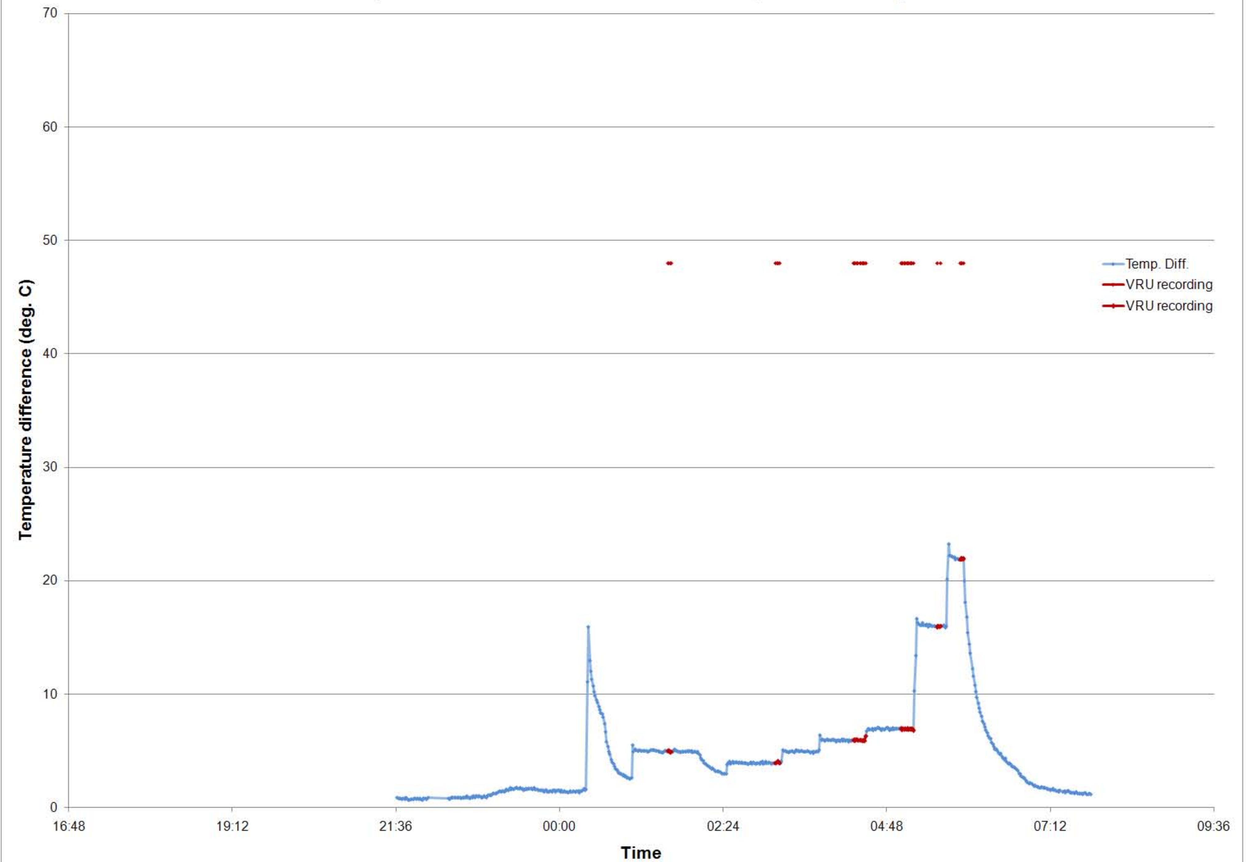
MEIS2-15 Temperatrure difference between HD and CD, VRU recording
