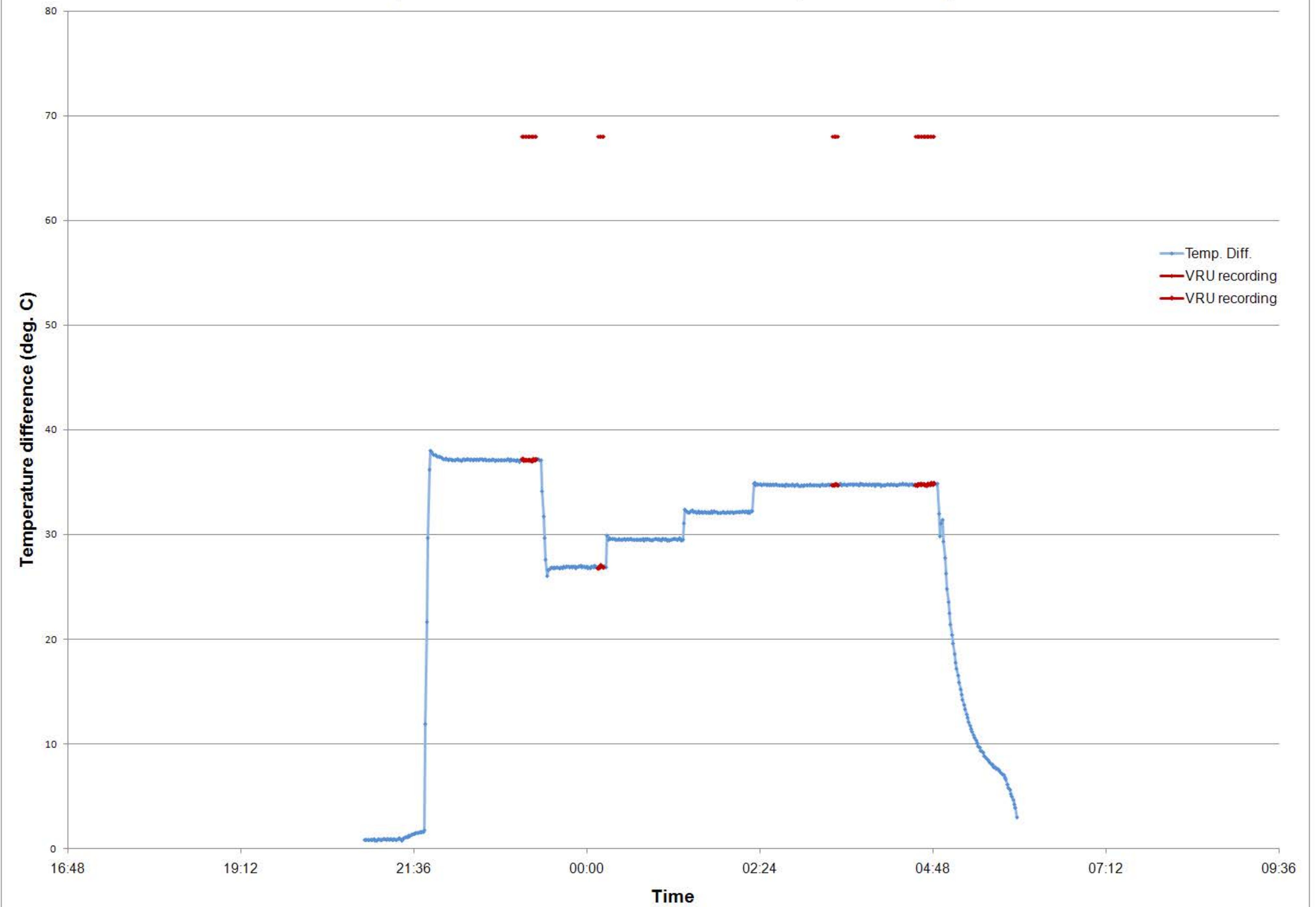
MEIS4-10 Temperatrure difference between HD and CD, VRU recording
