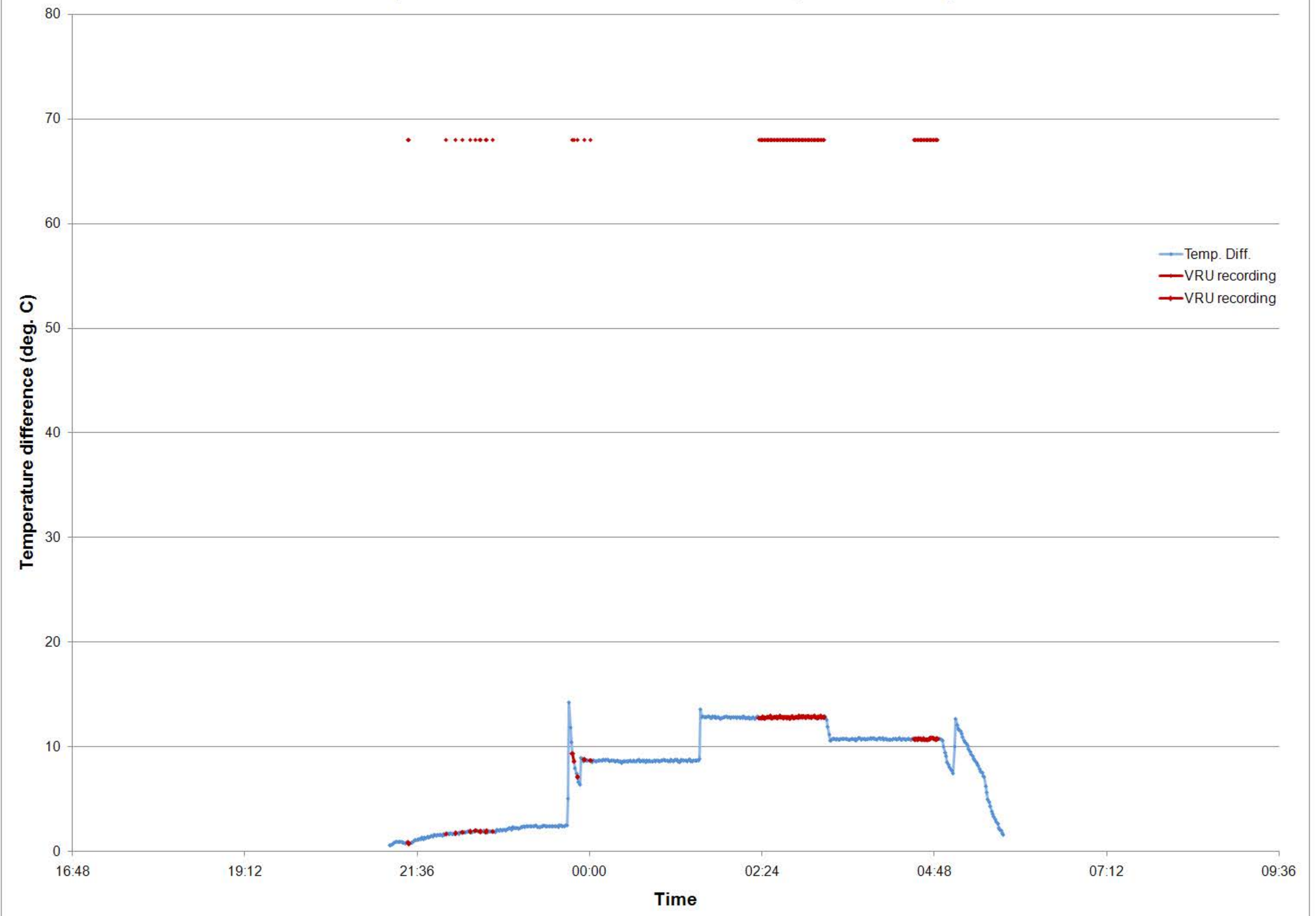
MEIS4-03 Temperatrure difference between HD and CD, VRU recording
