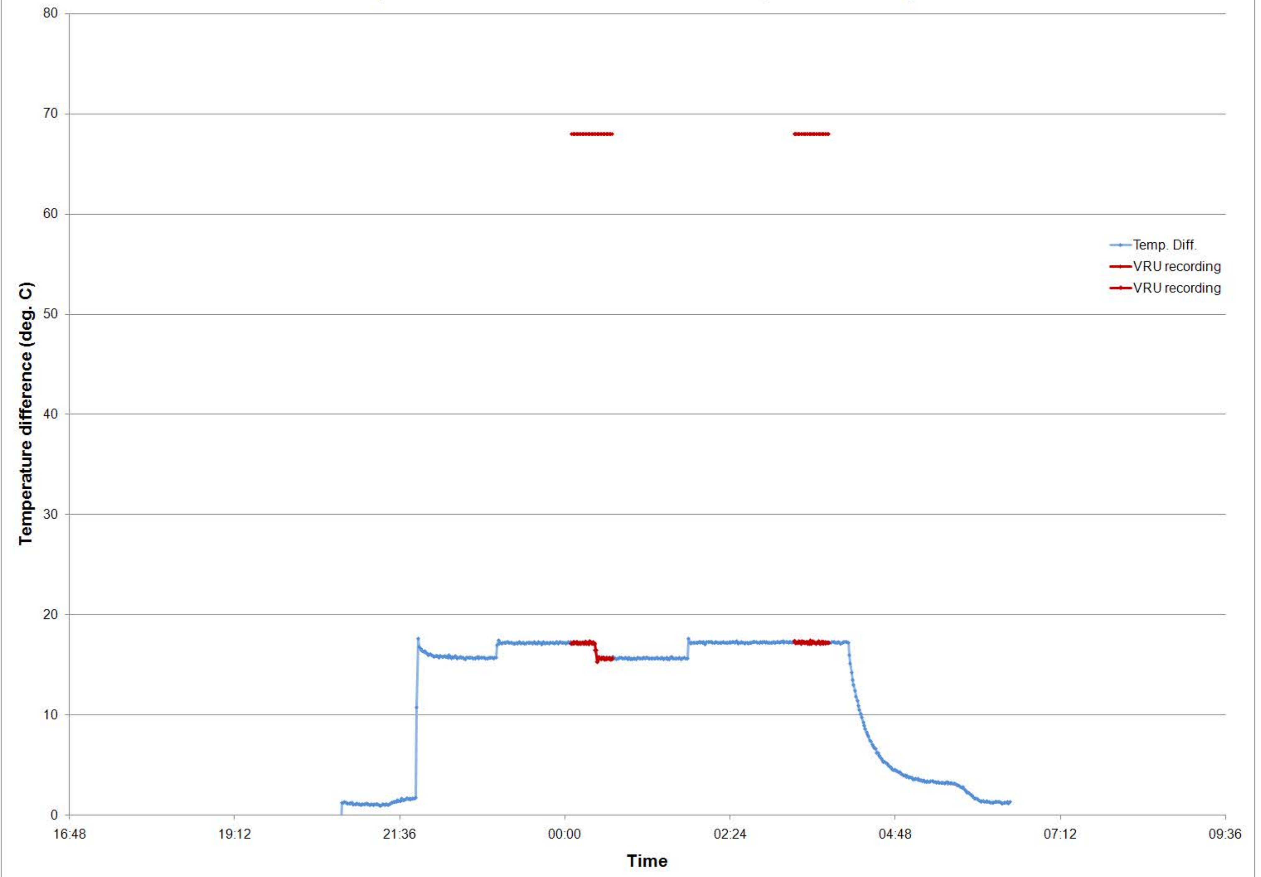
MEIS4-16 Temperatrure difference between HD and CD, VRU recording
