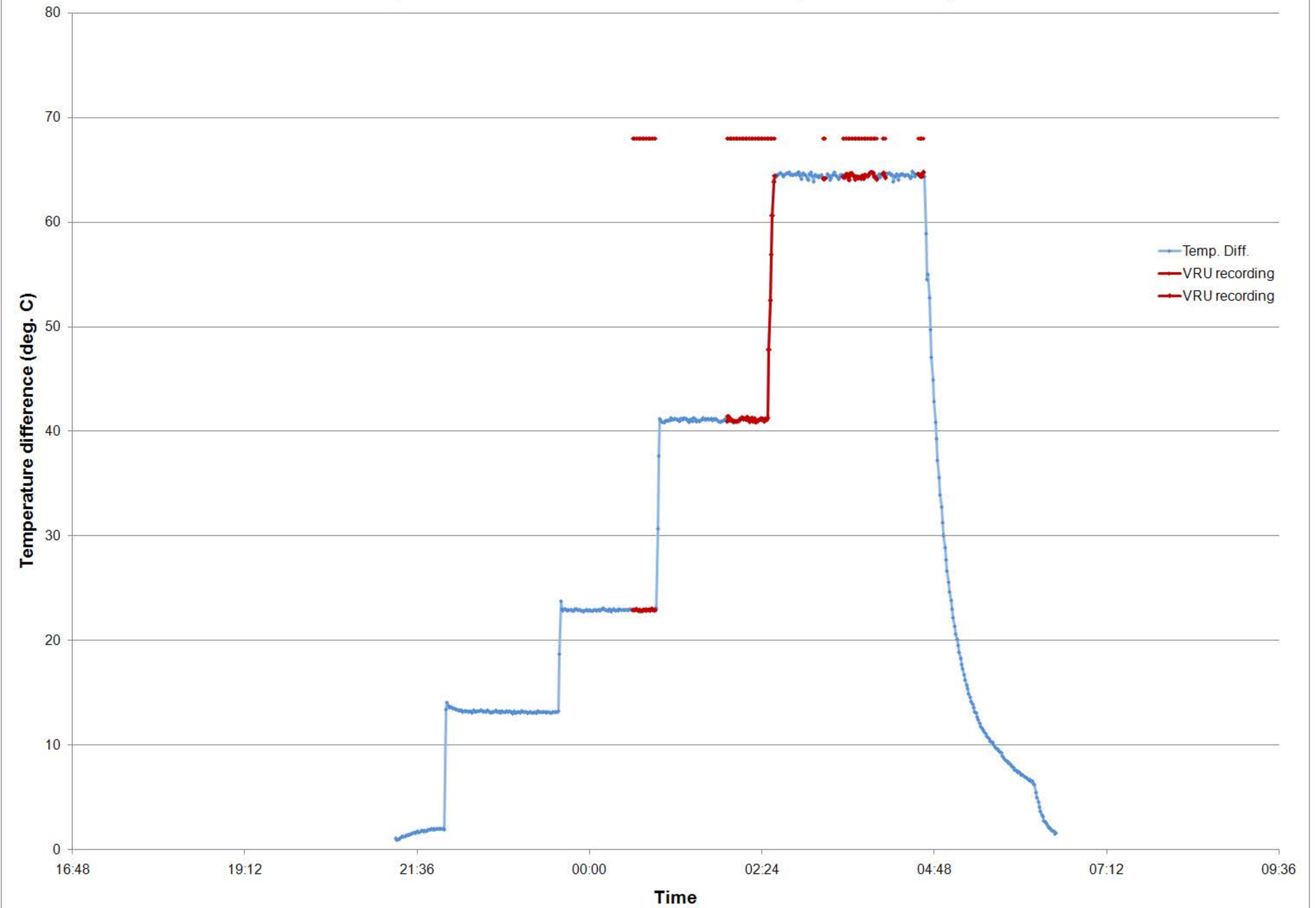
MEIS4-19 Temperatrure difference between HD and CD, VRU recording
