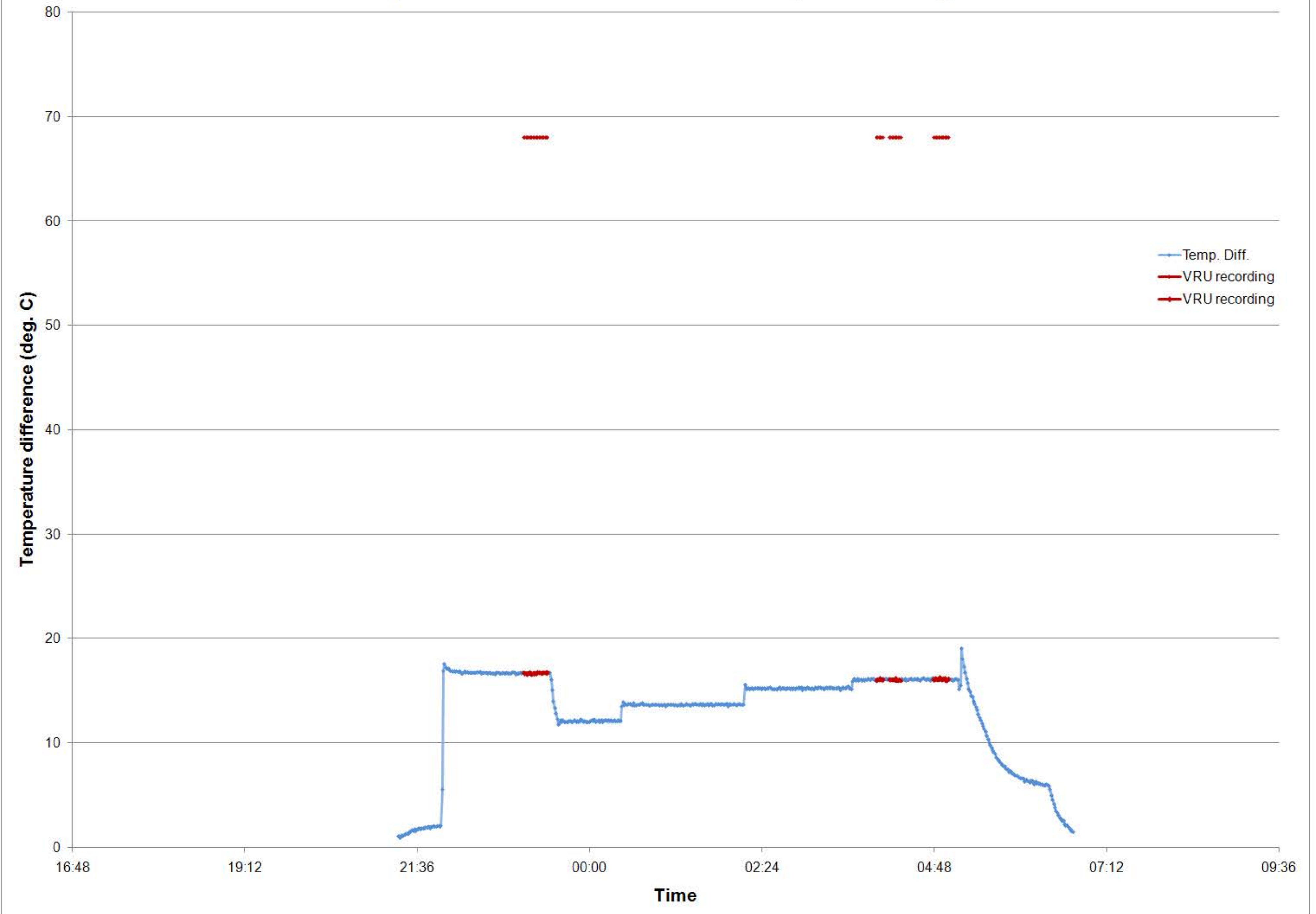
MEIS4-14 Temperatrure difference between HD and CD, VRU recording
