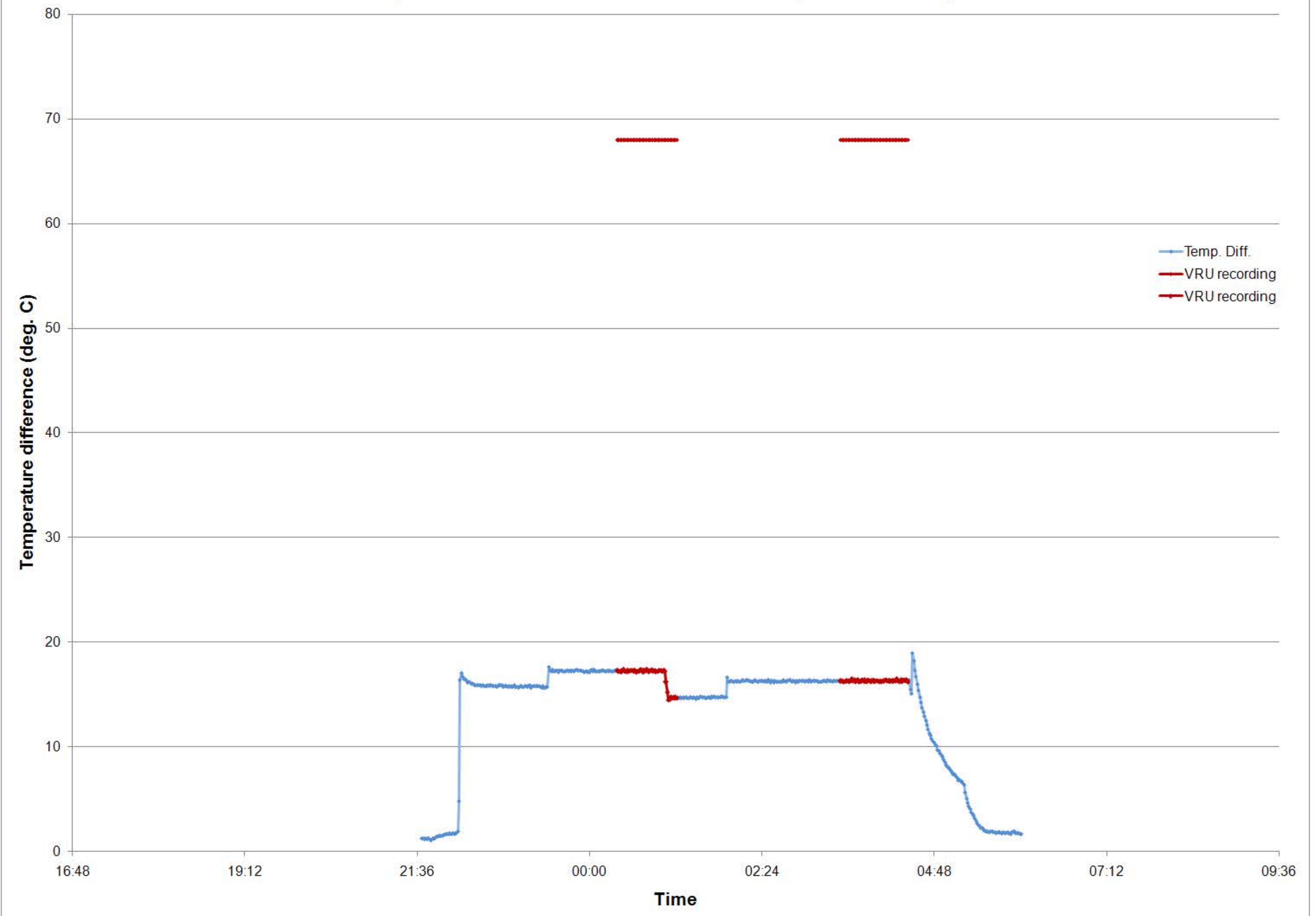
MEIS4-17 Temperatrure difference between HD and CD, VRU recording
