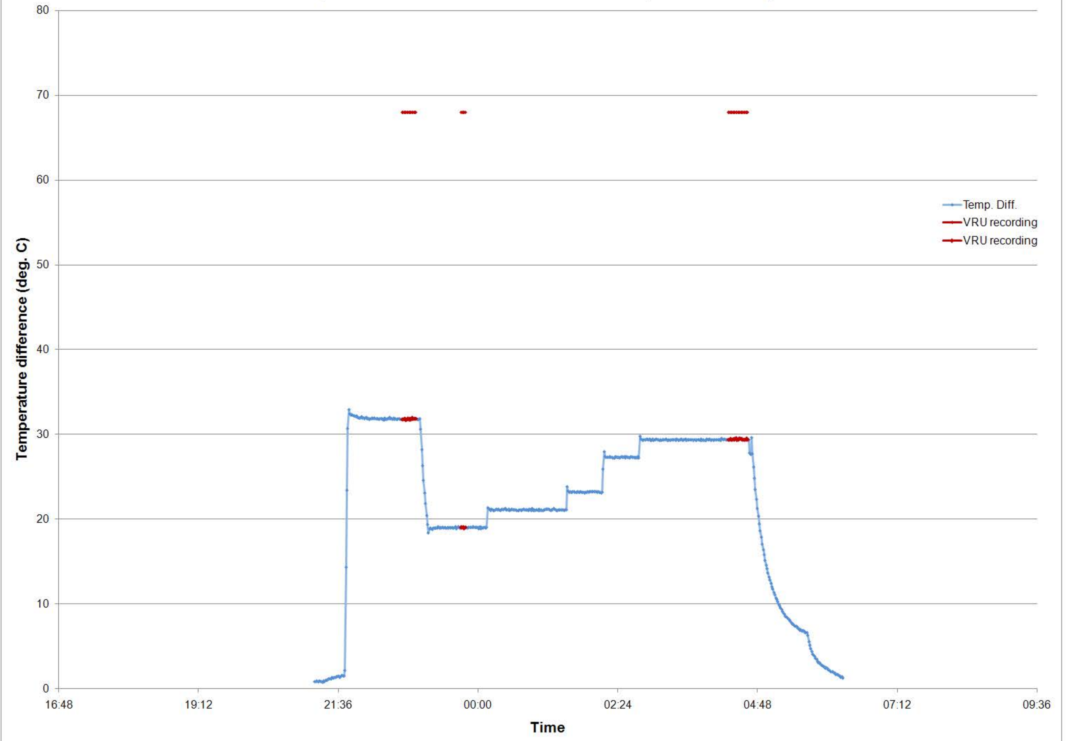
MEIS4-09 Temperatrure difference between HD and CD, VRU recording
