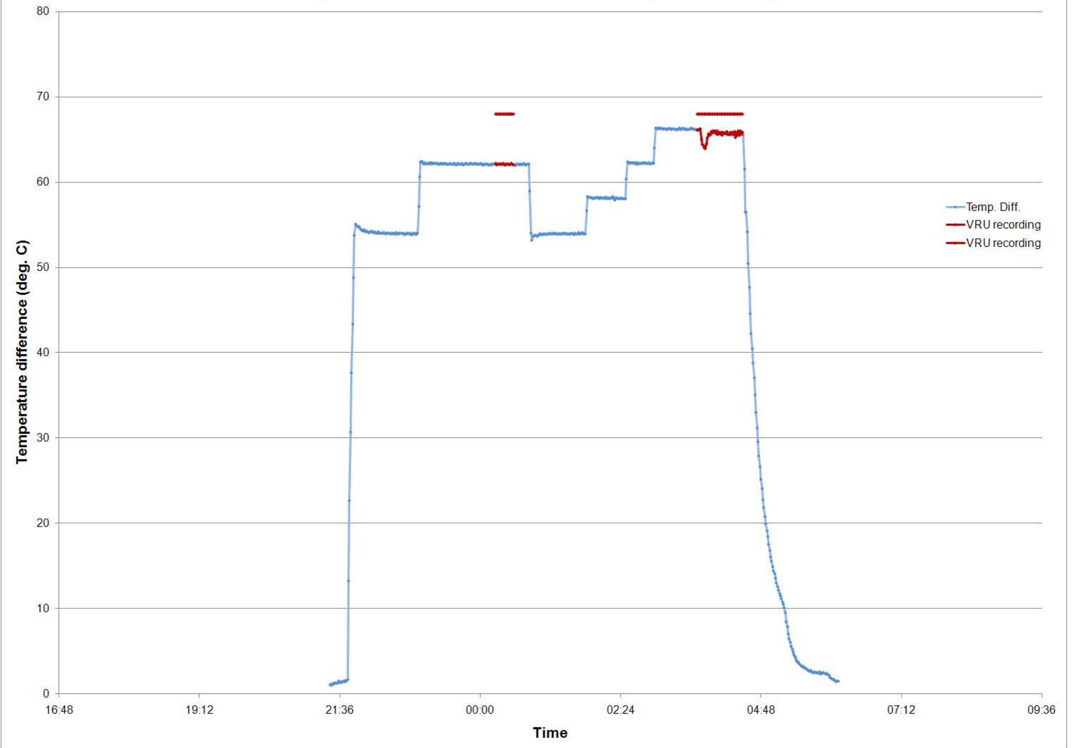
MEIS4-24 Temperatrure difference between HD and CD, VRU recording
