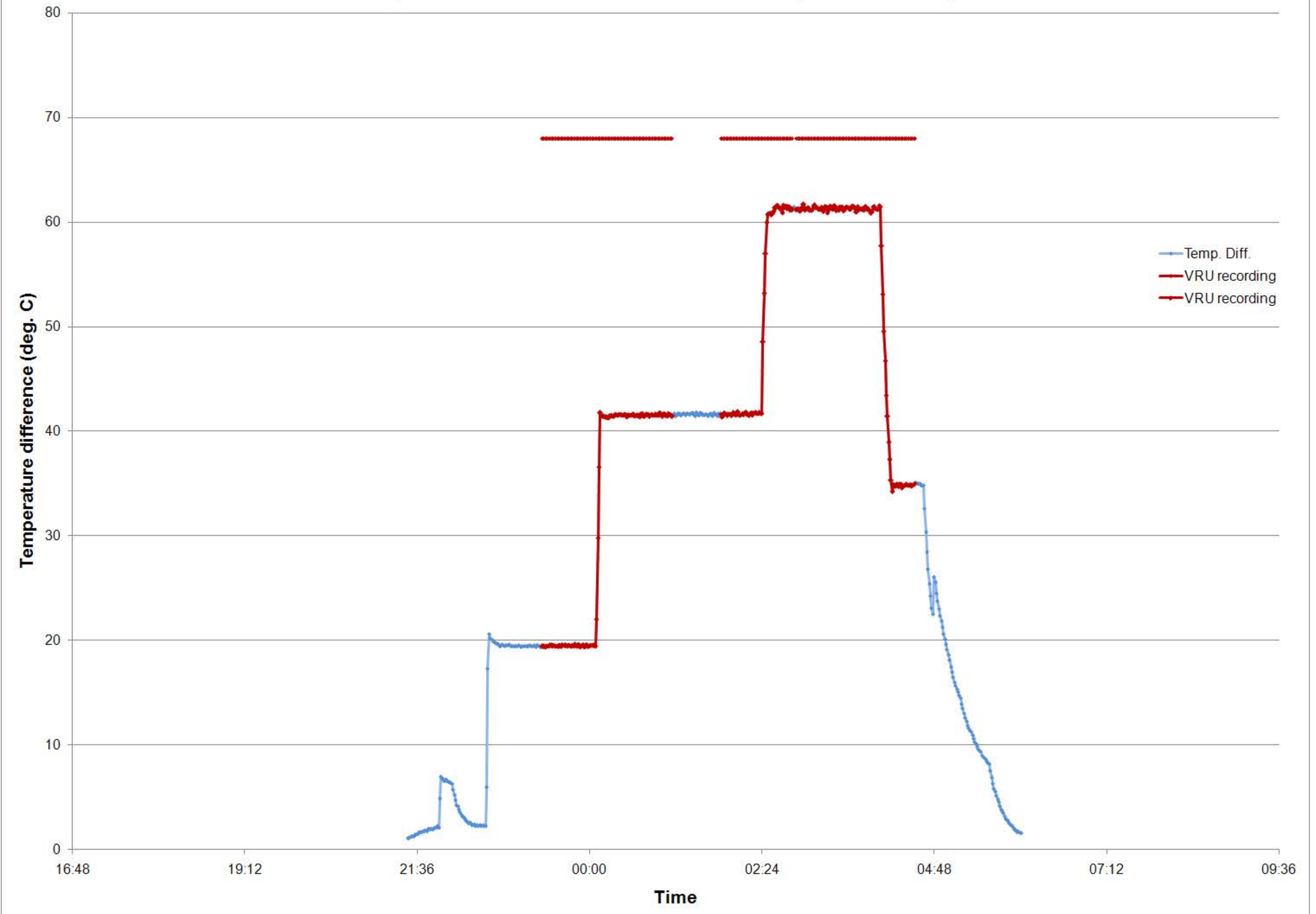
MEIS4-23 Temperatrure difference between HD and CD, VRU recording
