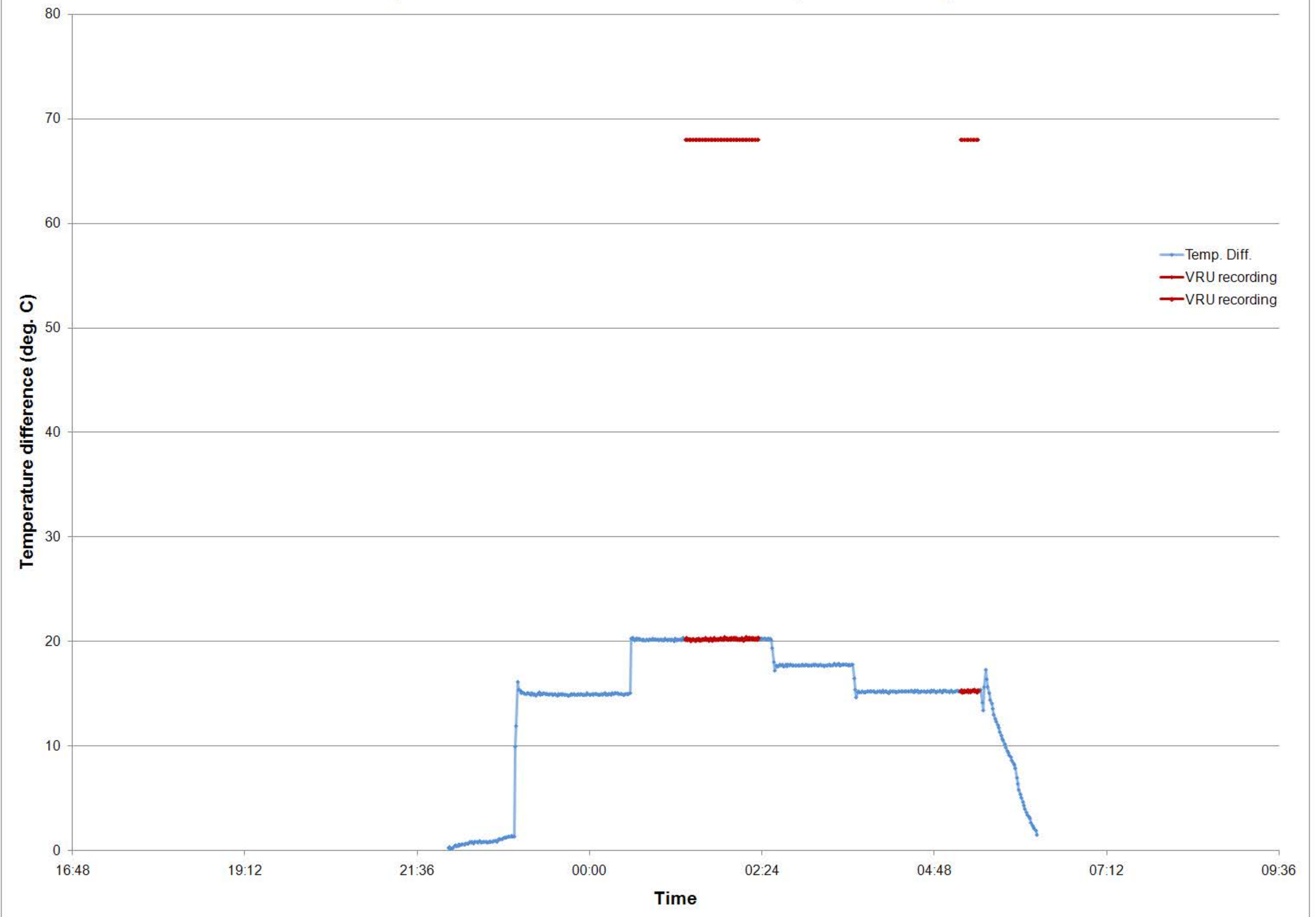
MEIS4-01 Temperatrure difference between HD and CD, VRU recording
