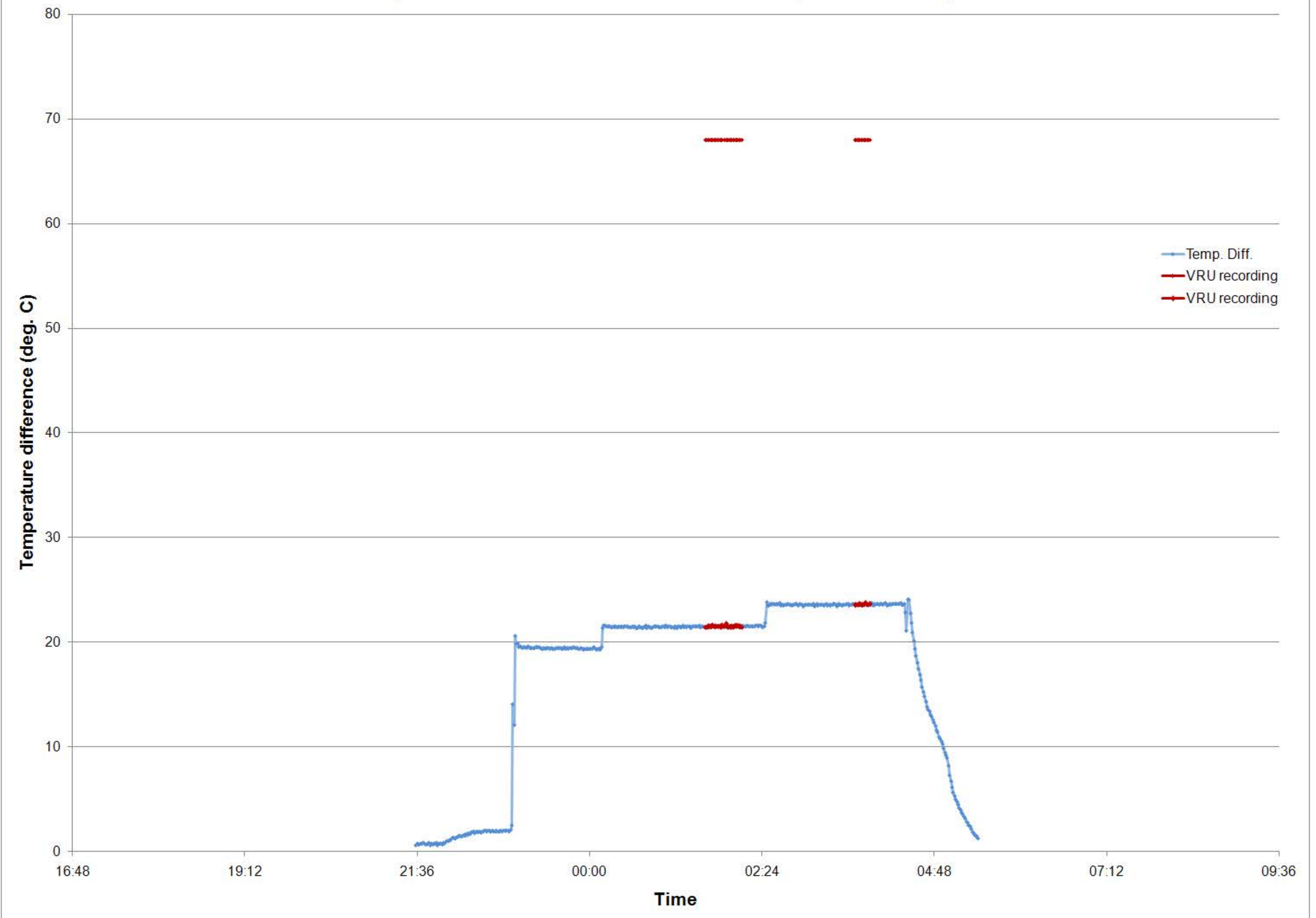
MEIS4-06 Temperatrure difference between HD and CD, VRU recording
