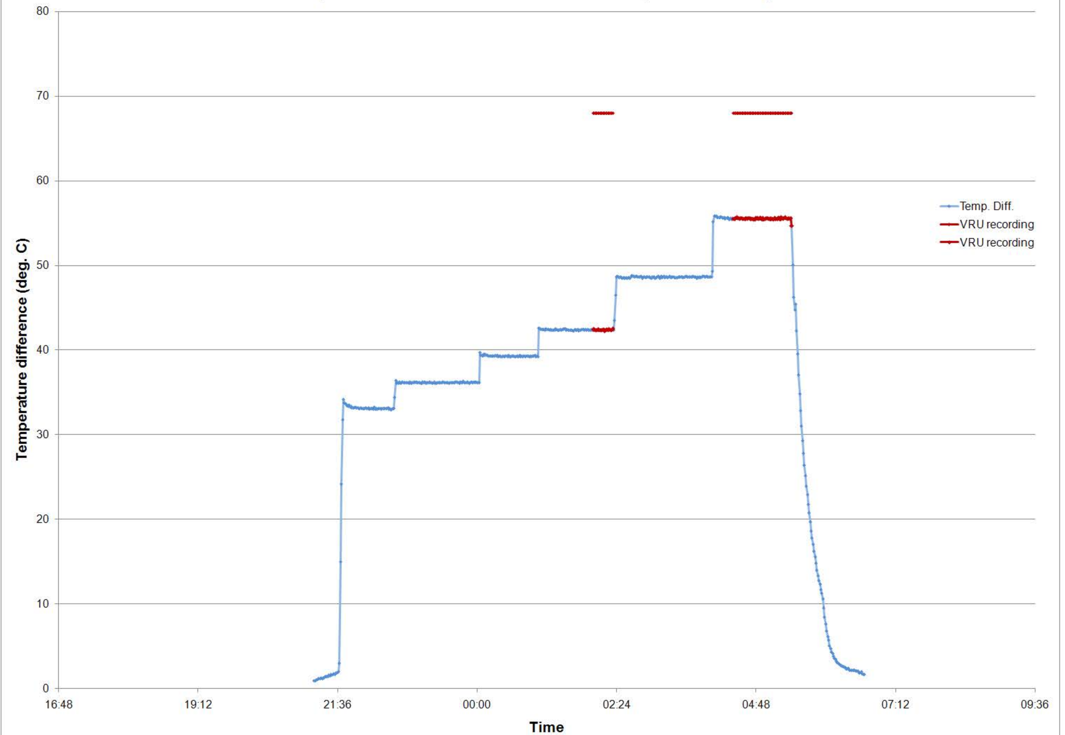
MEIS4-12 Temperatrure difference between HD and CD, VRU recording
