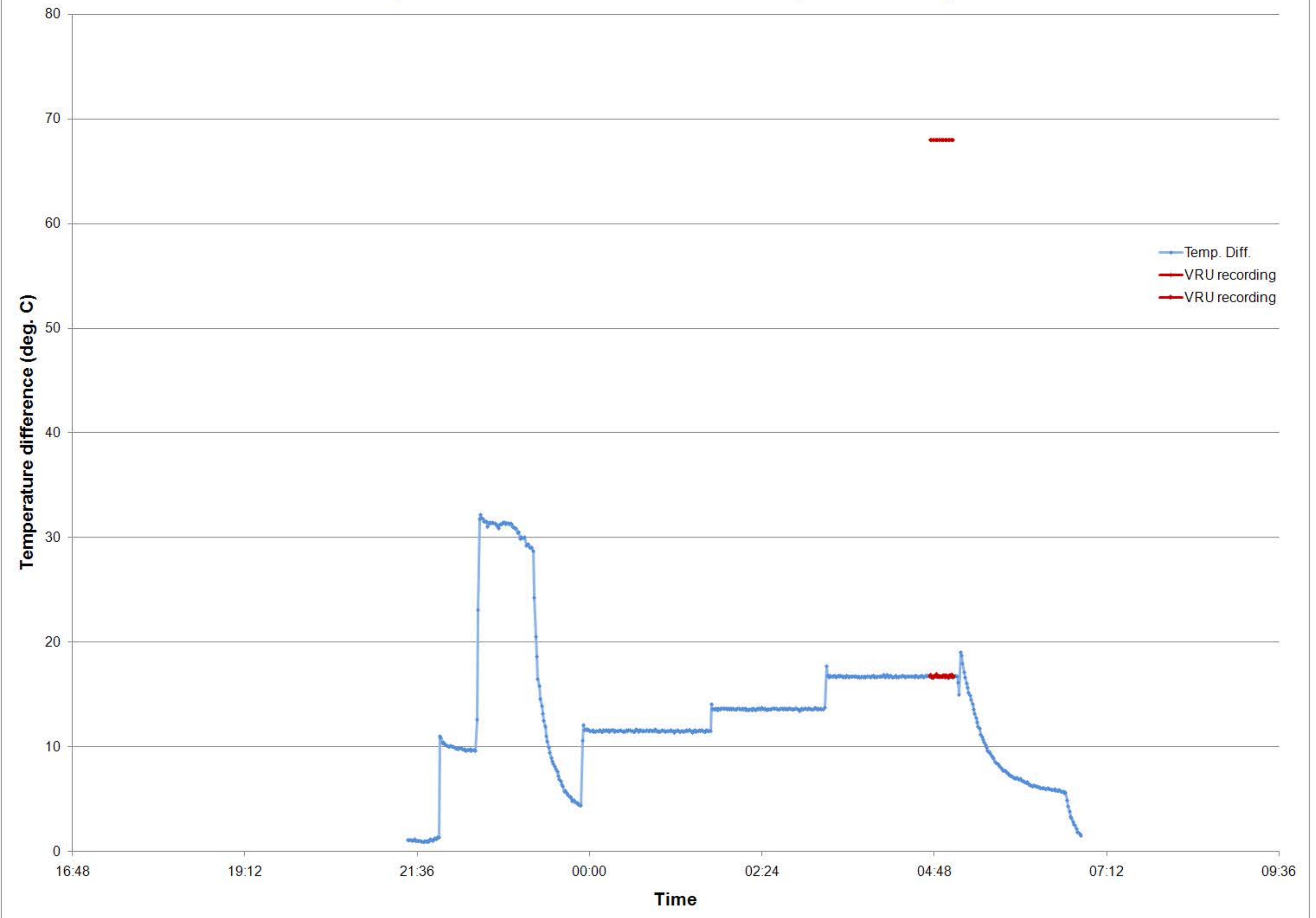
MEIS4-18 Temperatrure difference between HD and CD, VRU recording
