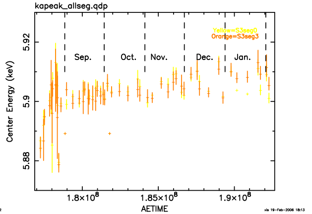
Figure 1: Center energy of the ^{55}\text{Fe} K- \alpha events after the CTI correction of rev. 1.0. as a function of the Astro-E time:(a) XIS0 (FI), (b) XIS1 (BI), (c) XIS2 (FI) and (d) XIS3.
