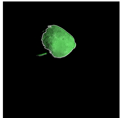
Figure 528: ST_2447904203_v.fits
