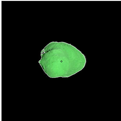
Figure 446: ST_2423411536_v.fits
