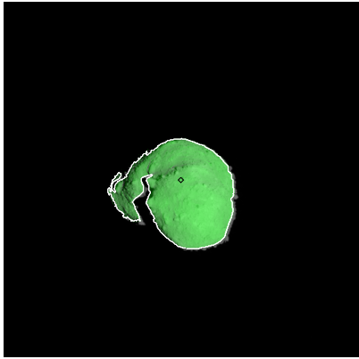
Figure 496: ST_2426270530_v.fits
