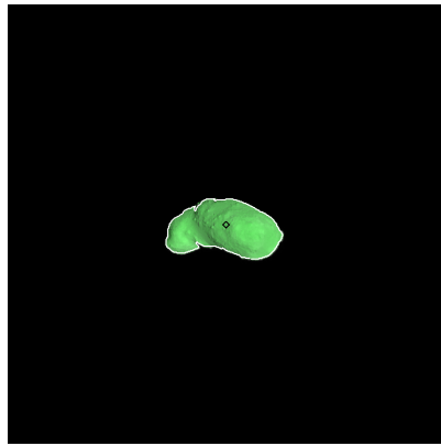
Figure 56: ST_2393634079_v.fits
