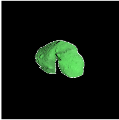
Figure 461: ST_2423534411_v.fits
