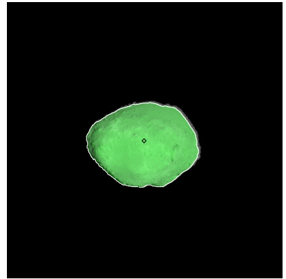
Figure 357: ST_2421322585_v.fits
