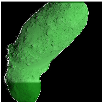
Figure 574: ST_2481672682_v.fits
