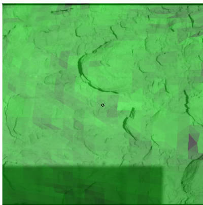
Figure 628: ST_2539451609_v.fits
