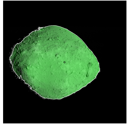
Figure 588: ST_2492513077_v.fits
