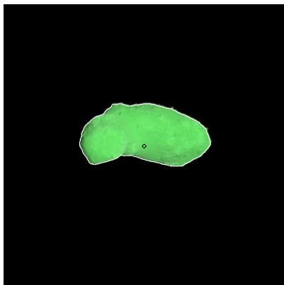
Figure 206: ST_2414876898_v.fits
