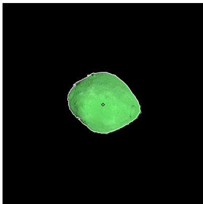
Figure 476: ST_2424165164_v.fits
