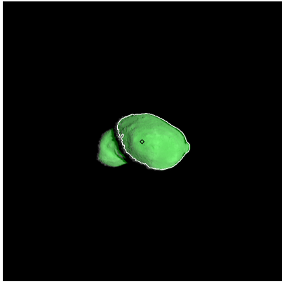
Figure 145: ST_2410307157_v.fits
