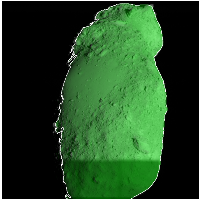
Figure 572: ST_2481211873_v.fits
