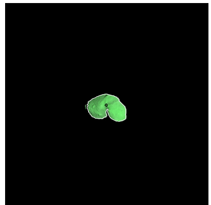
Figure 90: ST_2395645632_v.fits
