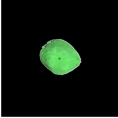
Figure 478: ST_2424181580_v.fits
