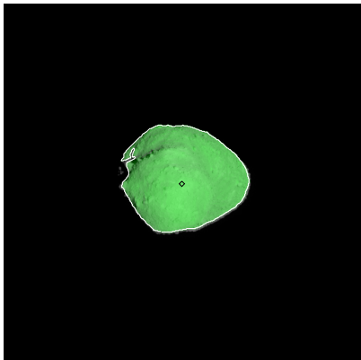
Figure 448: ST_2423427887_v.fits
