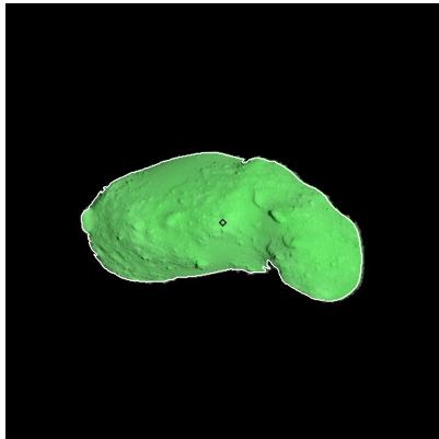
Figure 302: ST_2420872042_v.fits
