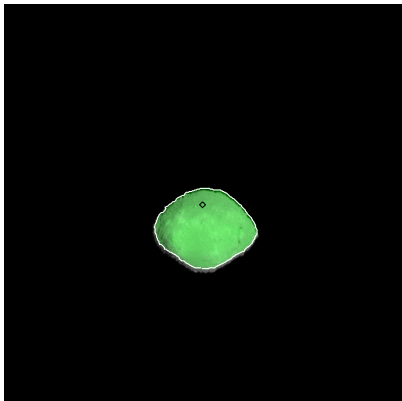
Figure 187: ST_2412972136_v.fits
