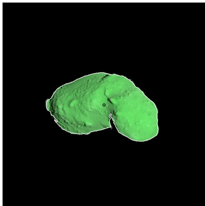
Figure 293: ST_2420798316_v.fits
