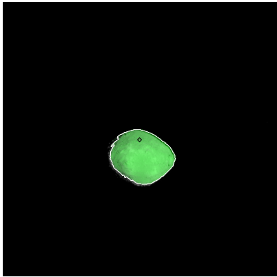
Figure 193: ST_2413018229_v.fits
