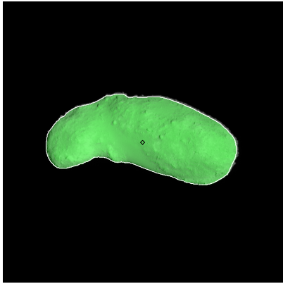
Figure 406: ST_2423083900_v.fits
