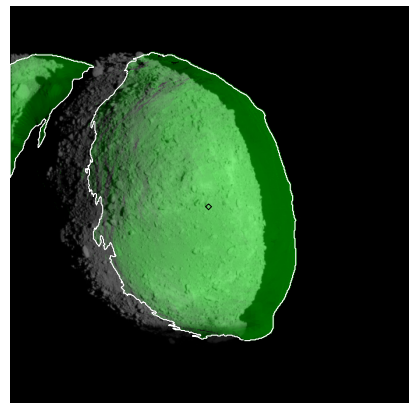
Figure 567: ST_2474500986_v.fits
