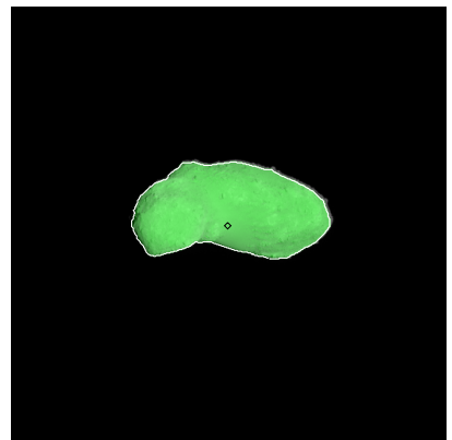
Figure 207: ST_2414884583_v.fits
