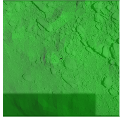
Figure 624: ST_2539423137_v.fits
