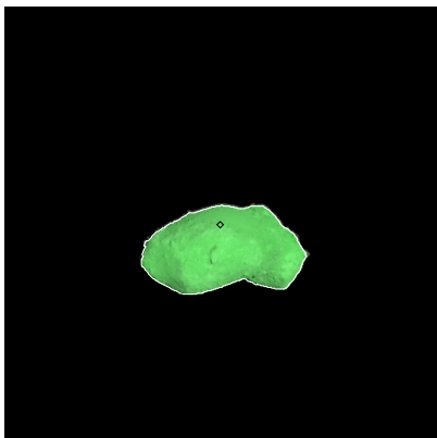
Figure 169: ST_2412833921_v.fits
