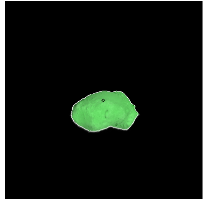
Figure 174: ST_2412872313_v.fits
