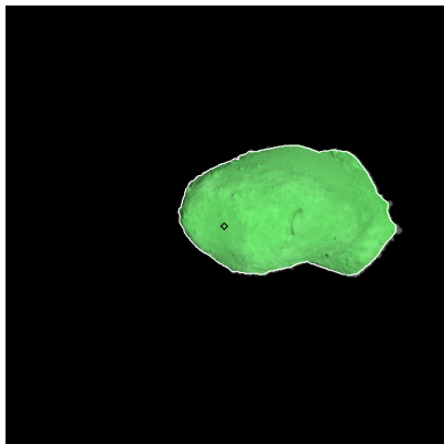
Figure 373: ST_2422649698_v.fits
