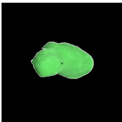
Figure 437: ST_2423337827_v.fits
