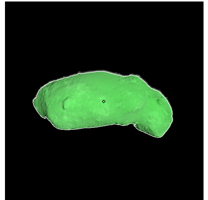
Figure 330: ST_2421101459_v.fits
