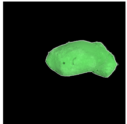
Figure 366: ST_2422592356_v.fits
