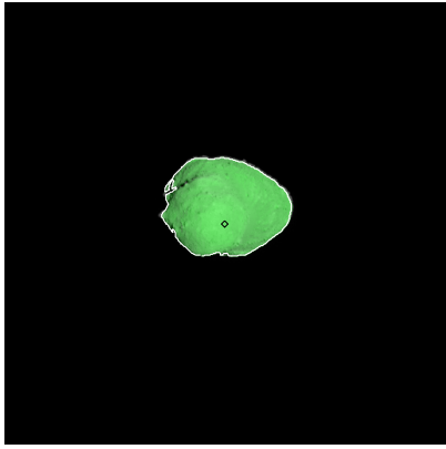
Figure 226: ST_2415030483_v.fits
