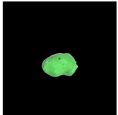
Figure 177: ST_2412895352_v.fits
