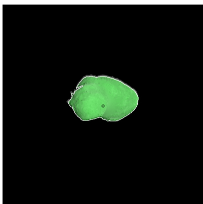
Figure 221: ST_2414992074_v.fits
