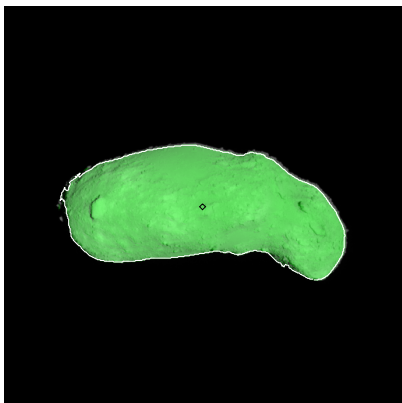
Figure 322: ST_2421035909_v.fits
