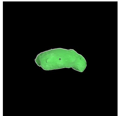
Figure 141: ST_240938528_v.fits
