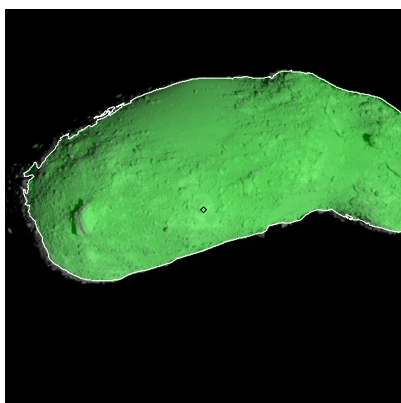
Figure 584: ST_2489465997_v.fits
