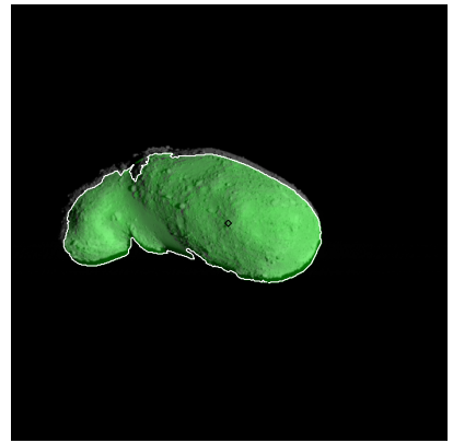
Figure 534: ST_2450874726_v.fits
