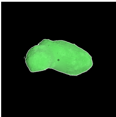
Figure 430: ST_2423280484_v.fits
