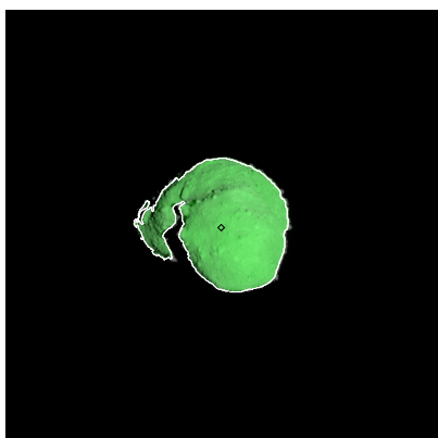
Figure 454: ST_2423477037_v.fits
