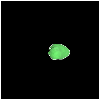
Figure 35: ST_2388513311_v.fits
