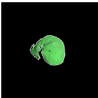
Figure 455: ST_2423485261_v.fits
