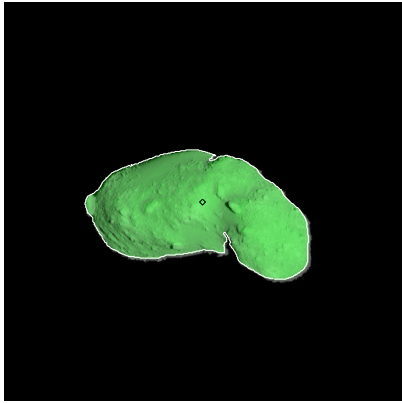
Figure 514: ST_2426418029_v.fits
