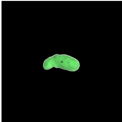
Figure 68: ST_2393726250_v.fits
