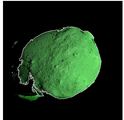
Figure 573: ST_2481442195_v.fits
