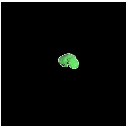
Figure 16: ST_2370516209_b.fits
