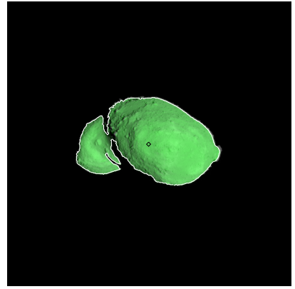
Figure 381: ST_2422879059_v.fits
