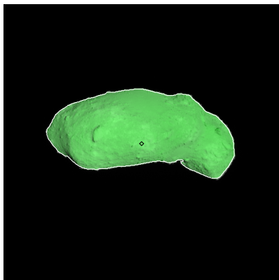
Figure 269: ST_2418699769_v.fits
