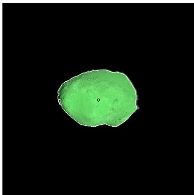
Figure 467: ST_2424091455_v.fits
