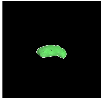
Figure 105: ST_2402958501_v.fits
