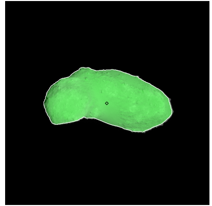
Figure 426: ST_2423247750_v.fits
