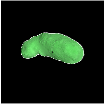
Figure 236: ST_2417420977_v.fits
