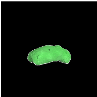
Figure 161: ST_2412734079_v.fits
