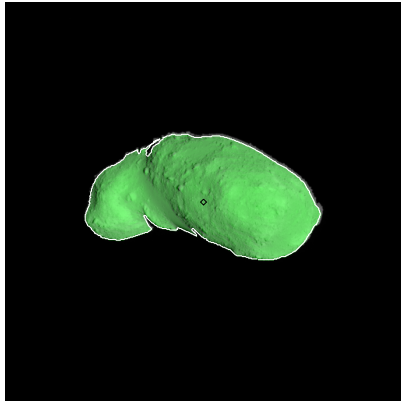
Figure 389: ST_2422944609_v.fits
