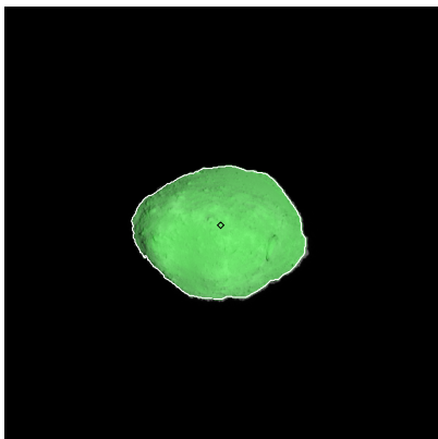
Figure 358: ST_2421330744_v.fits
