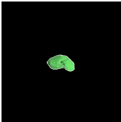
Figure 95: ST_2395684040_v.fits
