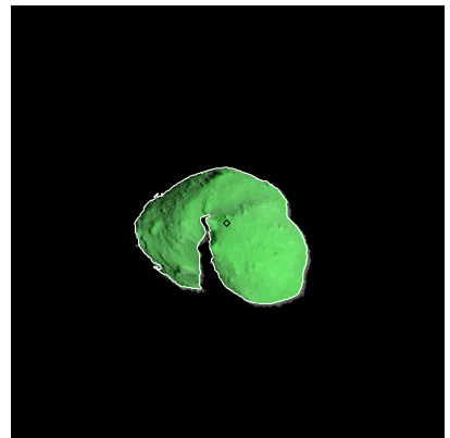
Figure 501: ST_2426311505_v.fits
