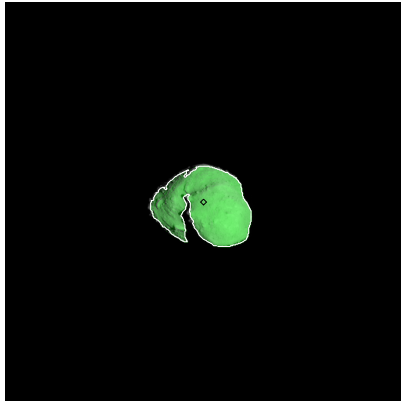
Figure 137: ST_2409546772_v.fits
