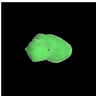
Figure 439: ST_2423354210_v.fits
