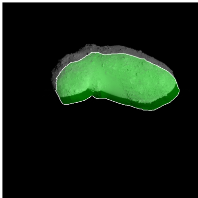
Figure 535: ST_2451105131_v.fits
