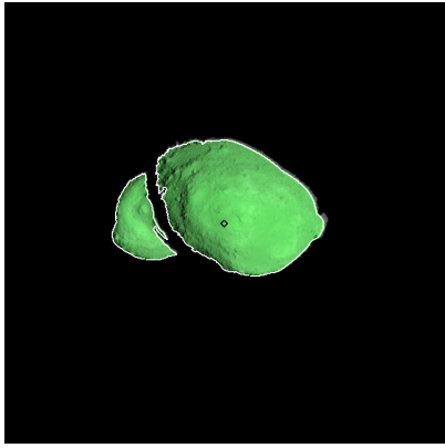
Figure 379: ST_2422862675_v.fits
