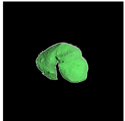
Figure 285: ST_2420732749_v.fits
