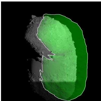
Figure 565: ST_2473604354_v.fits
