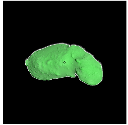
Figure 300: ST_2420855658_v.fits
