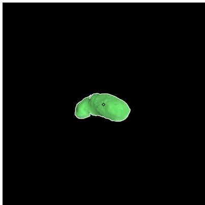
Figure 58: ST_2393649449_v.fits
