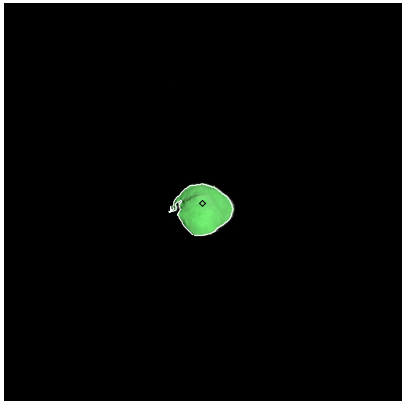
Figure 76: ST_2395530442_v.fits
