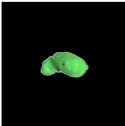
Figure 152: ST_2410360919_v.fits
