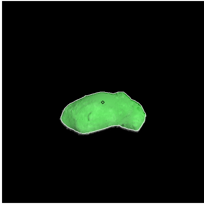
Figure 163: ST_2412787844_v.fits
