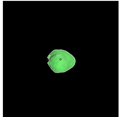
Figure 132: ST_2409469968_v.fits
