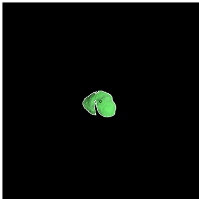
Figure 85: ST_2395599557_v.fits
