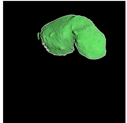
Figure 276: ST_2419381121_v.fits
