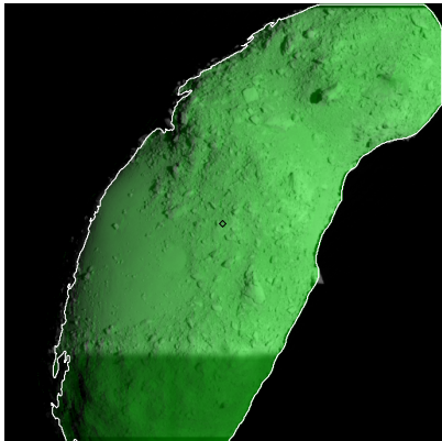
Figure 571: ST_2480981469_v.fits
