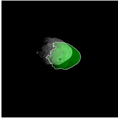
Figure 524: ST_2445698045_v.fits
