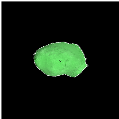
Figure 464: ST_2424066880_v.fits
