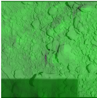
Figure 616: ST_2539429953_v.fits
