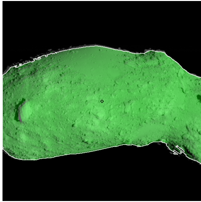
Figure 587: ST_2492225173_v.fits
