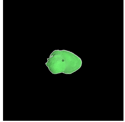
Figure 129: ST_2409423899_v.fits
