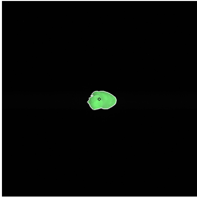
Figure 1: ST_2367541069_v.fits
