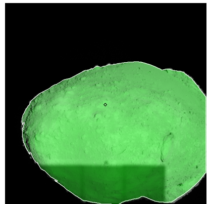
Figure 594: ST_2495287635_v.fits
