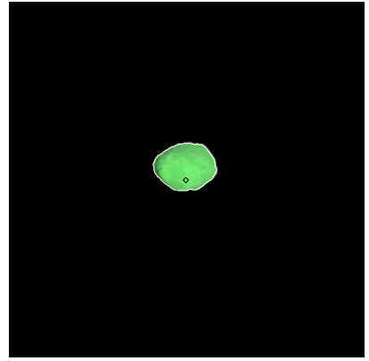
Figure 120: ST_2403179301_v.fits
