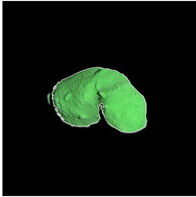
Figure 290: ST_2420773724_v.fits
