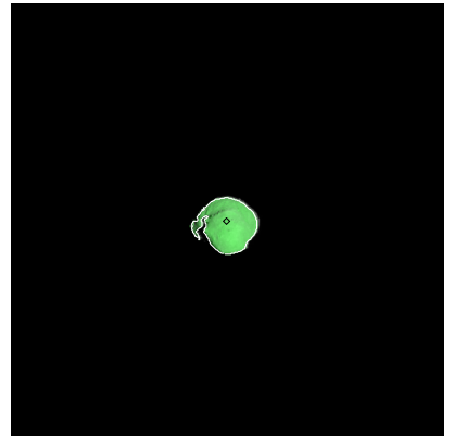
Figure 78: ST_2395545795_v.fits
