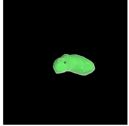
Figure 30: ST_2388369329_v.fits
