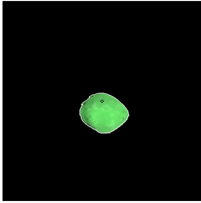
Figure 191: ST_2413002859_v.fits
