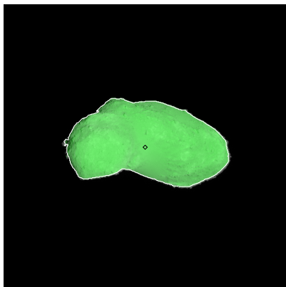
Figure 431: ST_2423288676_v.fits
