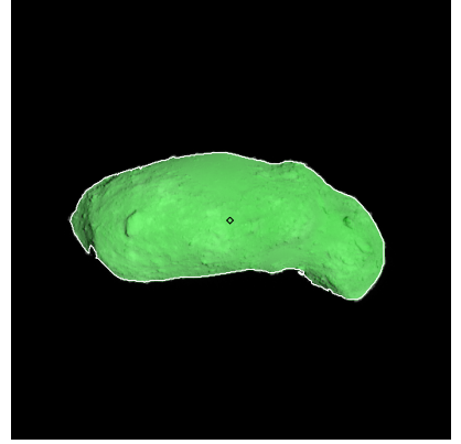
Figure 327: ST_2421076883_v.fits
