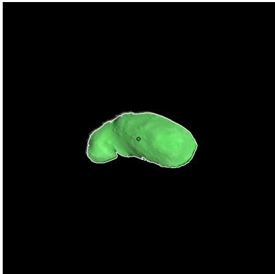
Figure 157: ST_2410399311_v.fits
