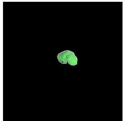
Figure 18: ST_2370593050_w.fits
