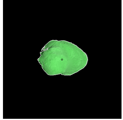
Figure 444: ST_2423395153_v.fits
