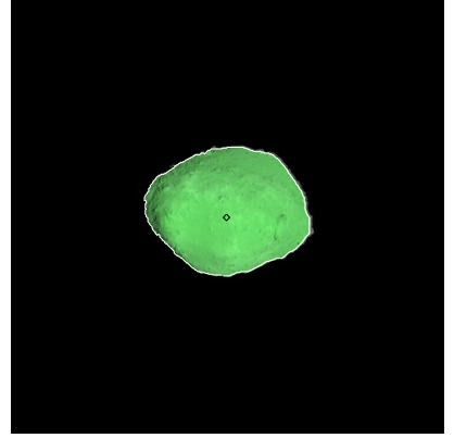
Figure 471: ST_2424124238_v.fits
