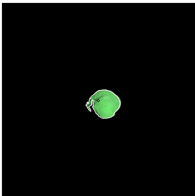
Figure 25: ST_2385775677_v.fits
