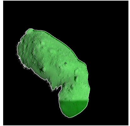
Figure 561: ST_2471117824_v.fits
