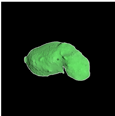
Figure 295: ST_2420814700_v.fits
