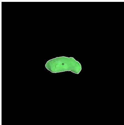
Figure 107: ST_2402996901_v.fits
