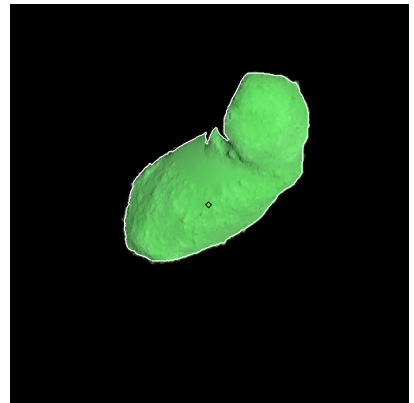
Figure 549: ST_2462414039_v.fits
