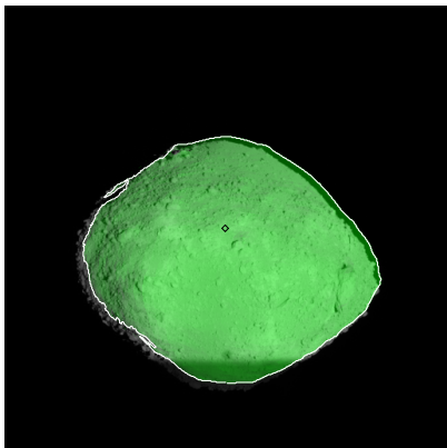
Figure 598: ST_2506502552_v.fits
