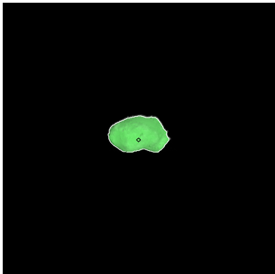
Figure 115: ST_2403112092_v.fits
