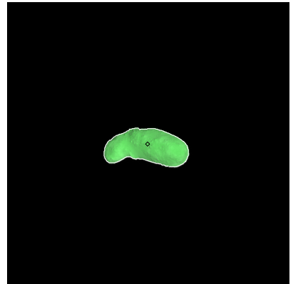
Figure 69: ST_2393733918_v.fits
