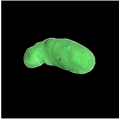
Figure 235: ST_2417413276_v.fits
