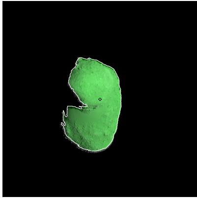
Figure 551: ST_2465255855_v.fits
