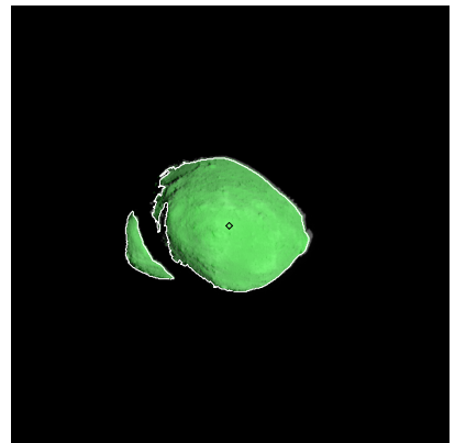
Figure 375: ST_2422829908_v.fits
