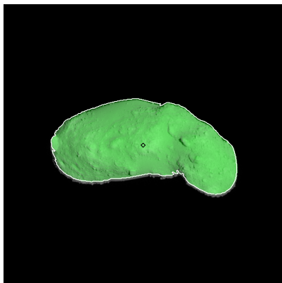
Figure 305: ST_2420896633_v.fits
