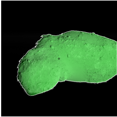
Figure 586: ST_2490253205_v.fits
