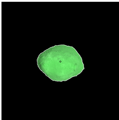
Figure 359: ST_2421338968_v.fits
