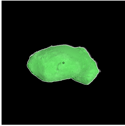
Figure 344: ST_2421216109_v.fits
