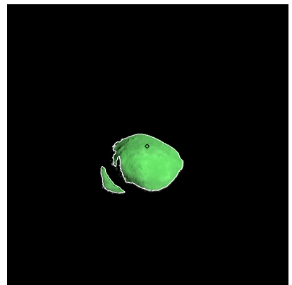
Figure 198: ST_2413056637_v.fits
