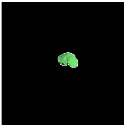
Figure 17: ST_2370554637_v.fits
