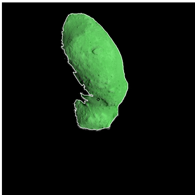
Figure 553: ST_2465906756_v.fits
