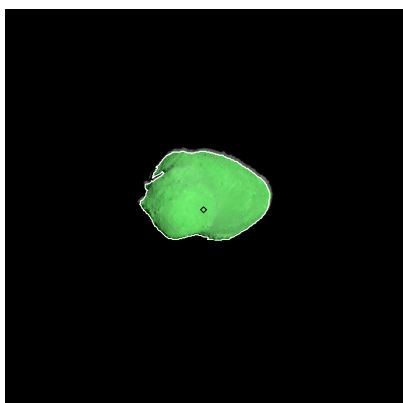
Figure 223: ST_2415007444_v.fits
