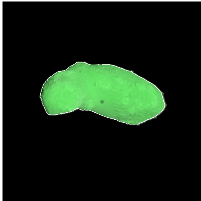
Figure 266: ST_2417651394_v.fits
