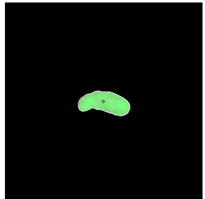
Figure 15: ST_2370439416_v.fits
