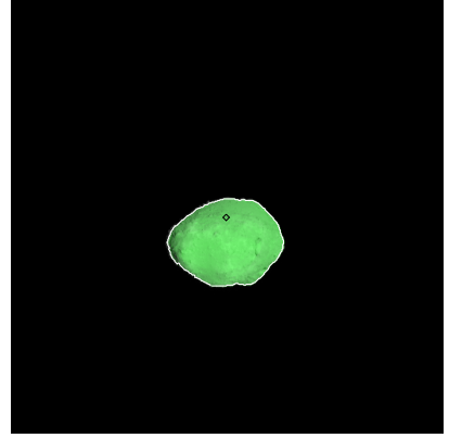
Figure 183: ST_2412941429_v.fits
