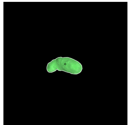
Figure 63: ST_2393687841_v.fits
