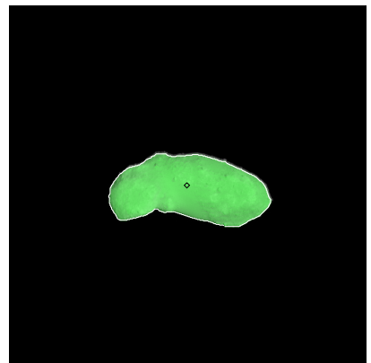
Figure 126: ST_2409239615_v.fits
