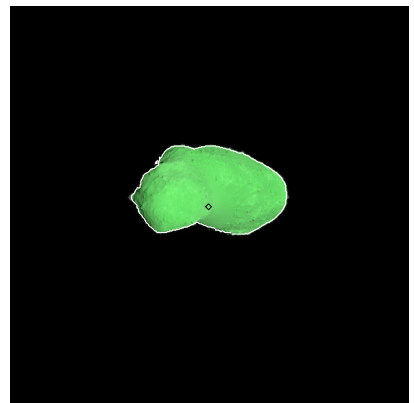
Figure 216: ST_2414953699_v.fits
