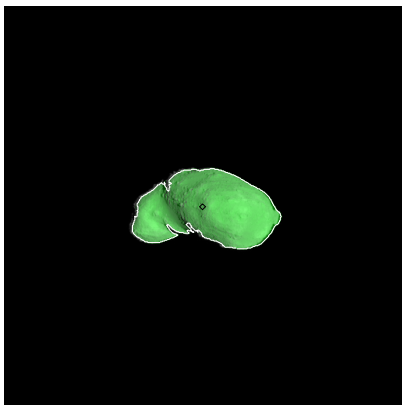
Figure 151: ST_2410353234_v.fits
