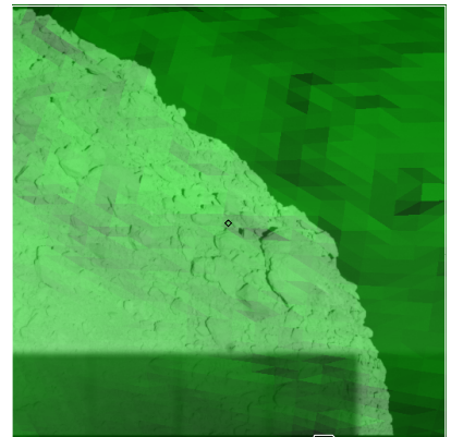
Figure 621: ST_2539482843_v.fits
