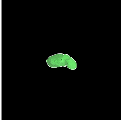
Figure 101: ST_2395730117_v.fits
