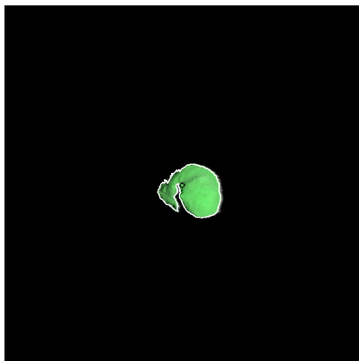
Figure 26: ST_2385806408_v.fits
