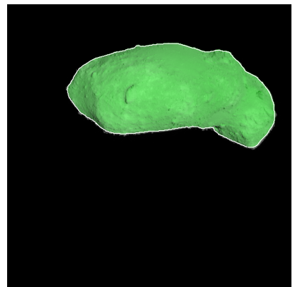
Figure 279: ST_2419745677_v.fits
