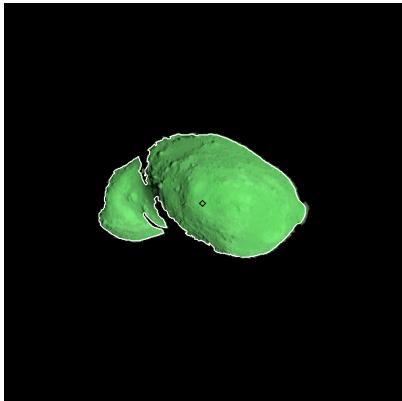
Figure 382: ST_2422887250_v.fits
