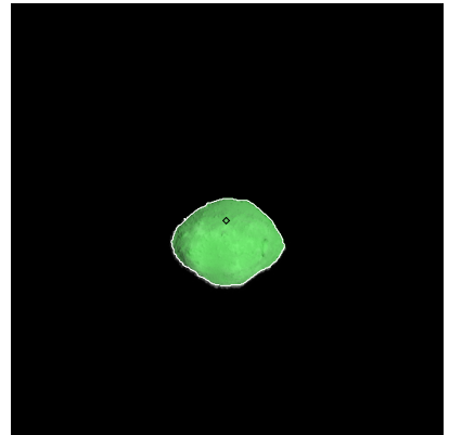
Figure 186: ST_2412964467_v.fits
