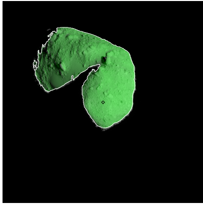
Figure 560: ST_2471012186_v.fits
