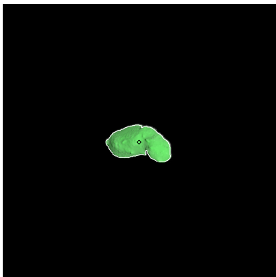
Figure 97: ST_2395699394_v.fits
