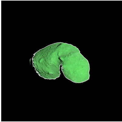
Figure 289: ST_2420765516_v.fits
