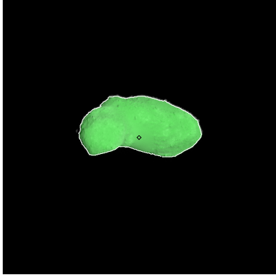
Figure 208: ST_2414892251_v.fits
