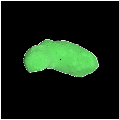
Figure 425: ST_2423239542_v.fits
