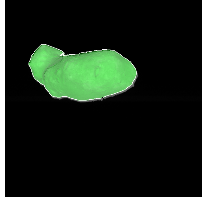
Figure 543: ST_2458929180_v.fits
