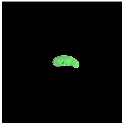
Figure 5: ST_2367977869_w.fits
