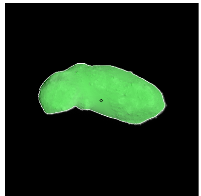
Figure 261: ST_2417613002_v.fits
