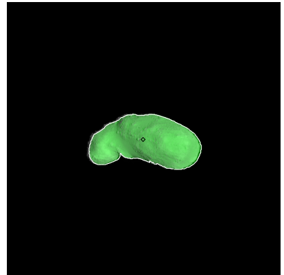
Figure 159: ST_2410414682_v.fits
