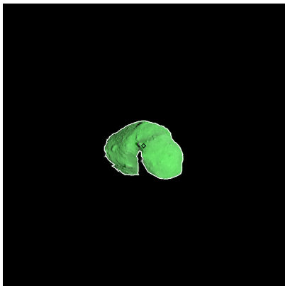
Figure 139: ST_2409577490_v.fits
