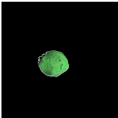
Figure 521: ST_2445006811_v.fits
