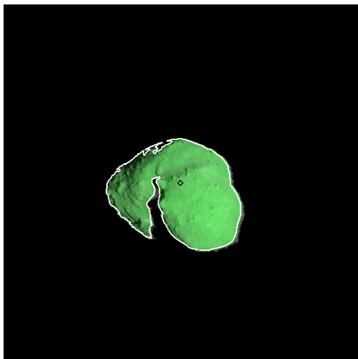
Figure 499: ST_2426295105_v.fits
