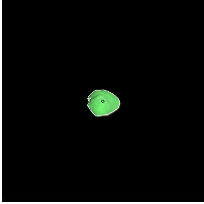
Figure 73: ST_2395507354_v.fits
