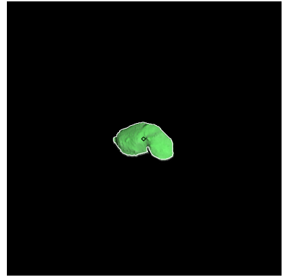
Figure 93: ST_2395668687_v.fits
