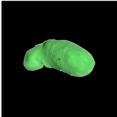
Figure 392: ST_2422969200_v.fits
