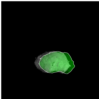
Figure 518: ST_2444259813_v.fits
