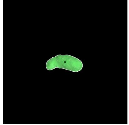
Figure 66: ST_2393710880_v.fits
