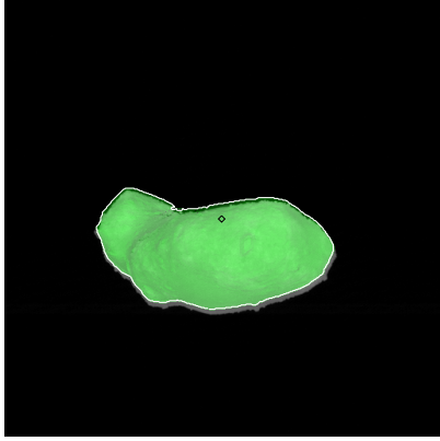
Figure 541: ST_2458542208_v.fits
