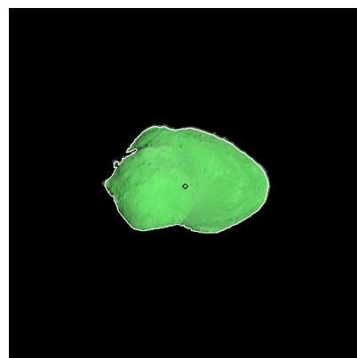
Figure 441: ST_2423370577_v.fits
