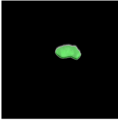
Figure 20: ST_2371015429_v.fits
