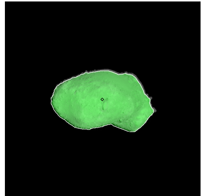
Figure 348: ST_2421248876_v.fits
