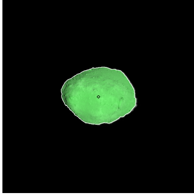
Figure 470: ST_2424116014_v.fits
