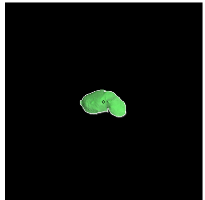
Figure 96: ST_2395691725_v.fits
