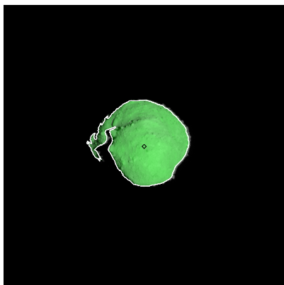
Figure 452: ST_2423460670_v.fits
