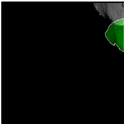
Figure 517: ST_2430878748_v.fits
