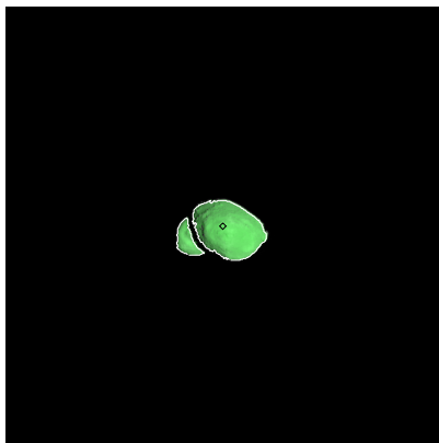
Figure 44: ST_2393541925_v.fits
