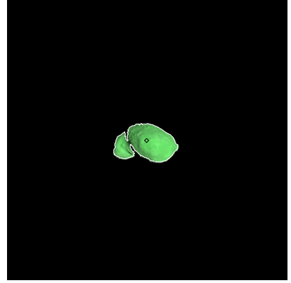
Figure 48: ST_2393572616_v.fits
