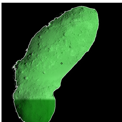
Figure 580: ST_2484583339_v.fits
