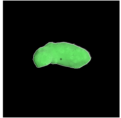
Figure 201: ST_2414838473_v.fits
