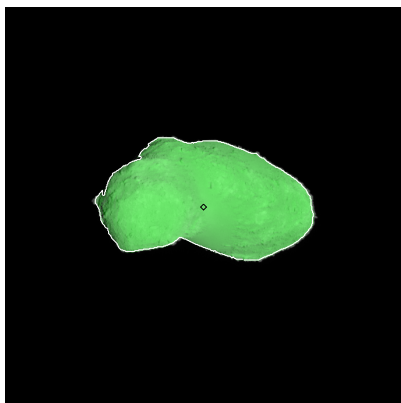
Figure 434: ST_2423313252_v.fits
