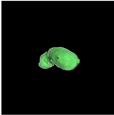
Figure 149: ST_2410337880_v.fits
