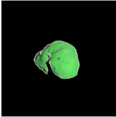
Figure 281: ST_2420699983_v.fits
