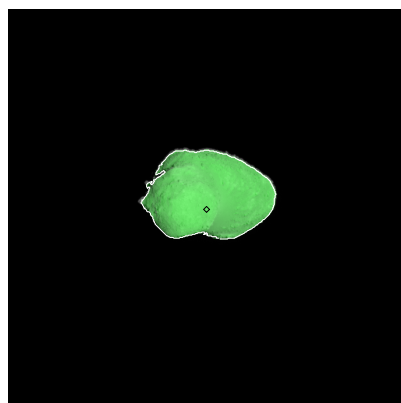
Figure 222: ST_2414999759_v.fits
