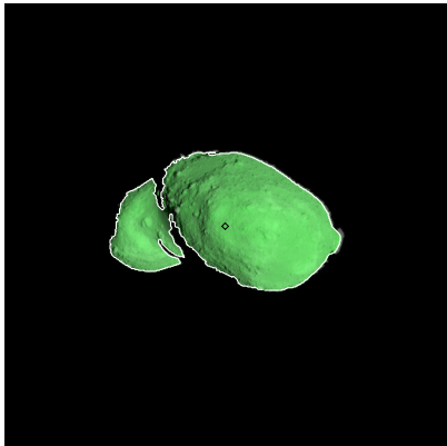
Figure 490: ST_2424279895_v.fits
