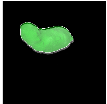
Figure 537: ST_2455809065_v.fits
