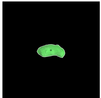
Figure 108: ST_2403006498_v.fits
