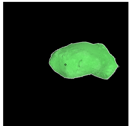
Figure 369: ST_2422616931_v.fits
