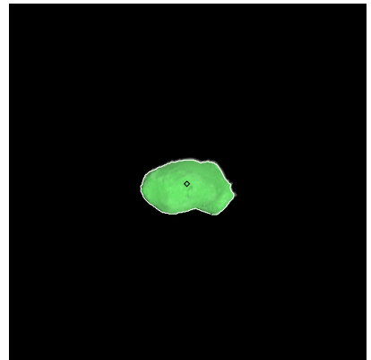
Figure 36: ST_2390548562_v.fits
