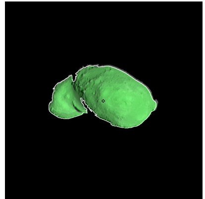
Figure 492: ST_2424296278_v.fits
