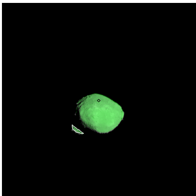
Figure 196: ST_2413041267_v.fits
