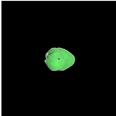
Figure 131: ST_2409454601_v.fits
