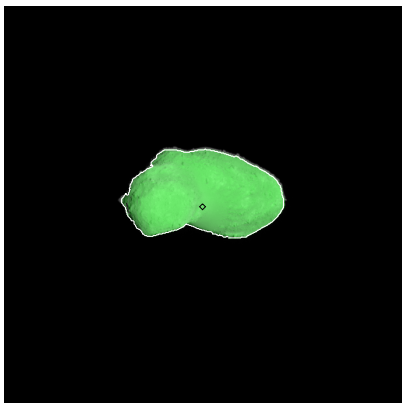
Figure 214: ST_2414938329_v.fits
