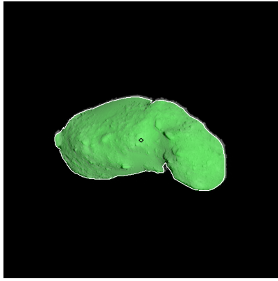
Figure 299: ST_2420847483_v.fits
