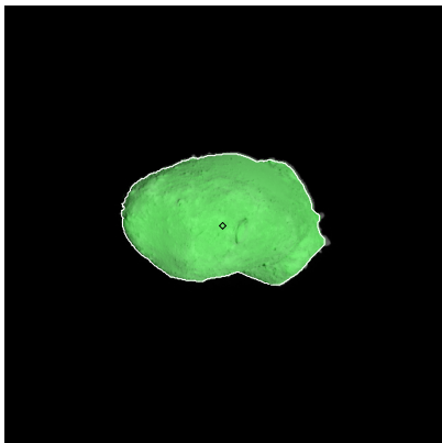
Figure 463: ST_2424058721_v.fits
