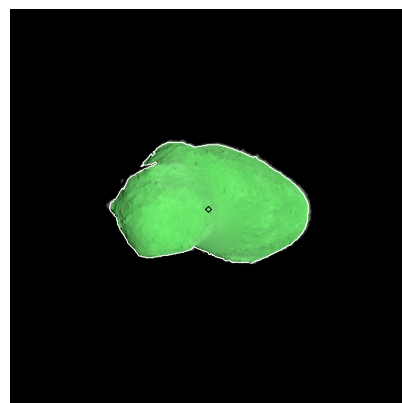
Figure 438: ST_2423346019_v.fits
