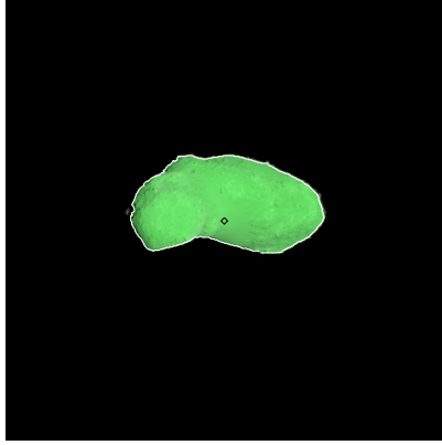
Figure 209: ST_2414899936_v.fits
