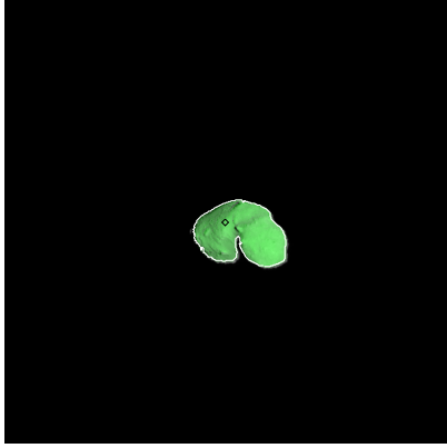
Figure 28: ST_2385864015_v.fits
