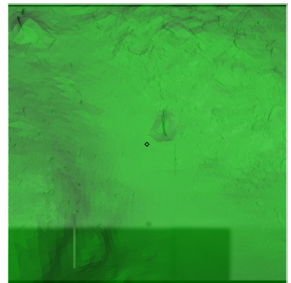
Figure 609: ST_2530292409_v.fits
