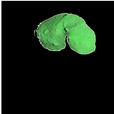
Figure 275: ST_2419372913_v.fits
