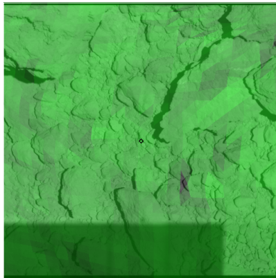
Figure 617: ST_2539437177_v.fits
