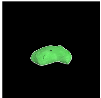
Figure 162: ST_2412780159_v.fits
