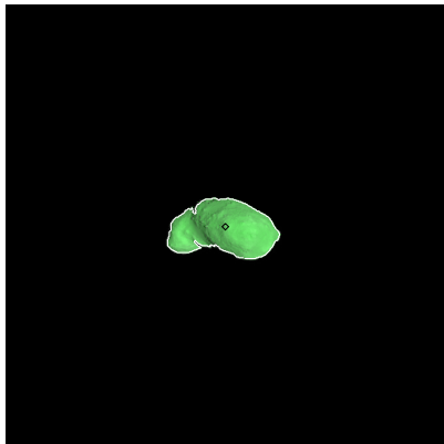
Figure 53: ST_2393611041_v.fits
