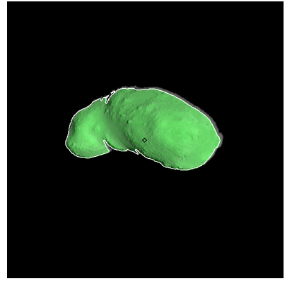
Figure 228: ST_2417359514_v.fits
