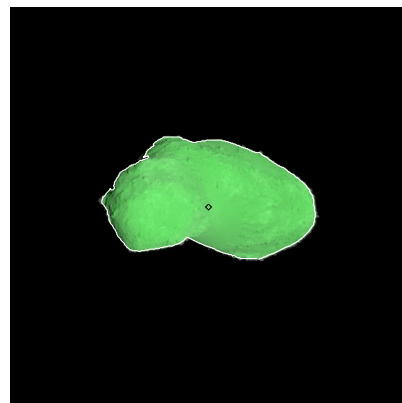
Figure 435: ST_2423321460_v.fits
