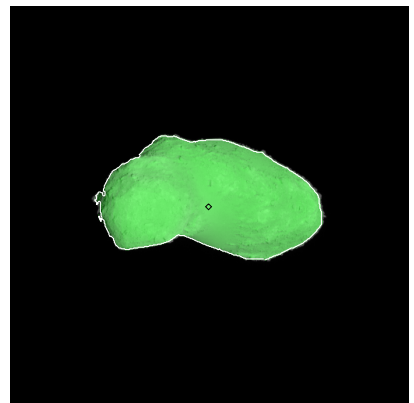
Figure 432: ST_2423296901_v.fits
