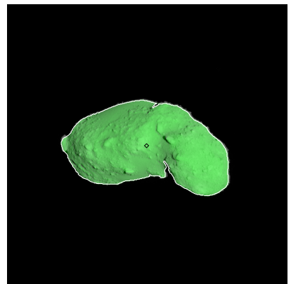
Figure 297: ST_2420831083_v.fits
