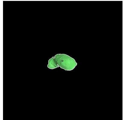
Figure 51: ST_2393595687_v.fits
