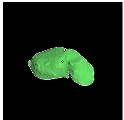
Figure 513: ST_2426409837_v.fits
