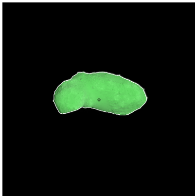
Figure 203: ST_2414853859_v.fits
