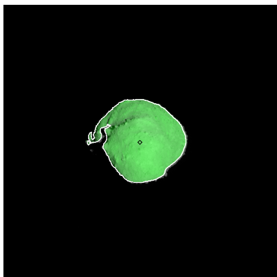
Figure 451: ST_2423452462_v.fits
