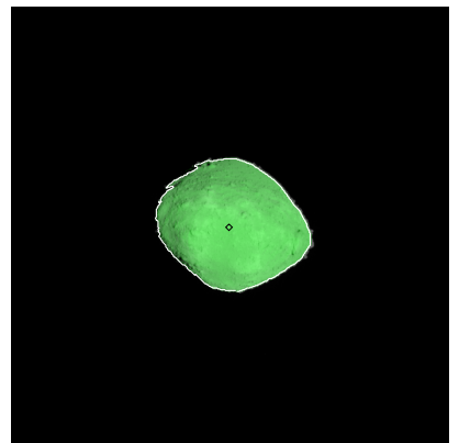
Figure 477: ST_2424173388_v.fits
