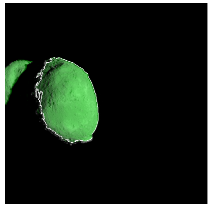
Figure 558: ST_2470301744_v.fits
