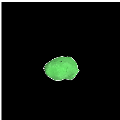
Figure 179: ST_2412910705_v.fits
