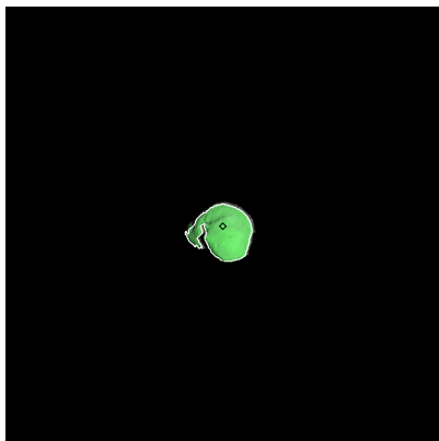
Figure 80: ST_2395561149_v.fits
