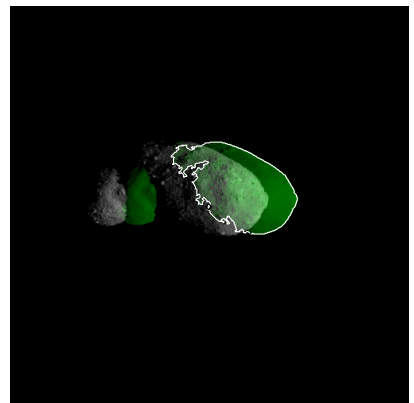
Figure 522: ST_2445206532_v.fits
