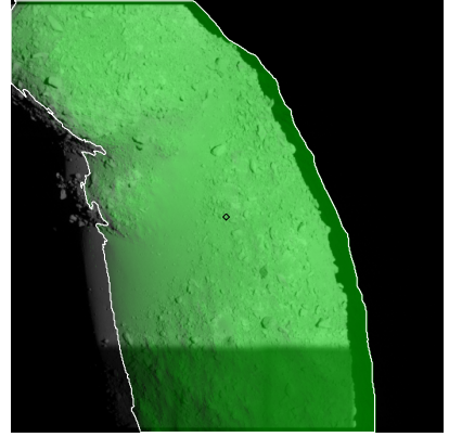
Figure 570: ST_2474846738_v.fits
