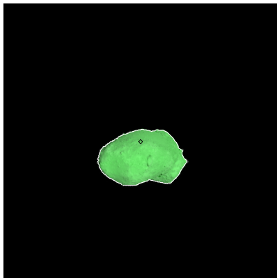
Figure 176: ST_2412887667_v.fits
