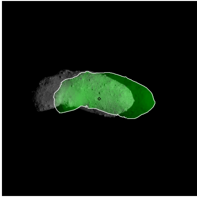
Figure 523: ST_2445692340_v.fits
