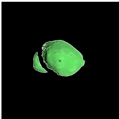
Figure 376: ST_2422838068_v.fits
